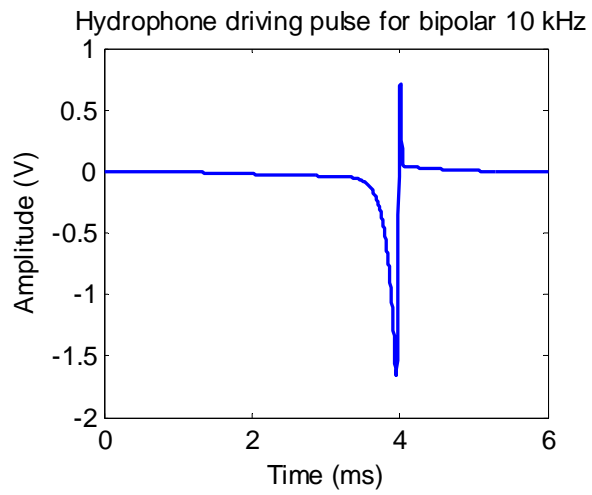
Figure 3.9 Input signal for hydrophone driving.
