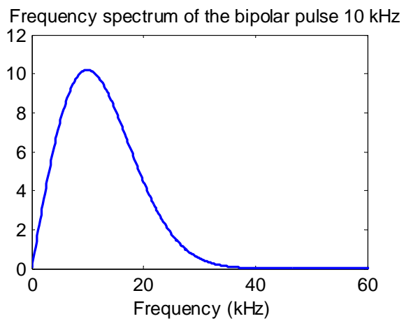
Figure 3.11 Frequency spectrum of the bipolar pulse 10 kHz.
