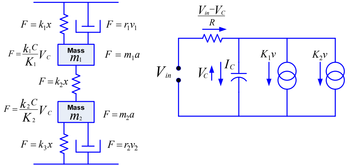
Figure 3.2 A simple model of a hydrophone.
