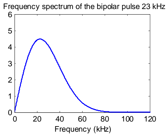
Figure 3.14 Frequency spectrum of the bipolar pulse 23 kHz.
