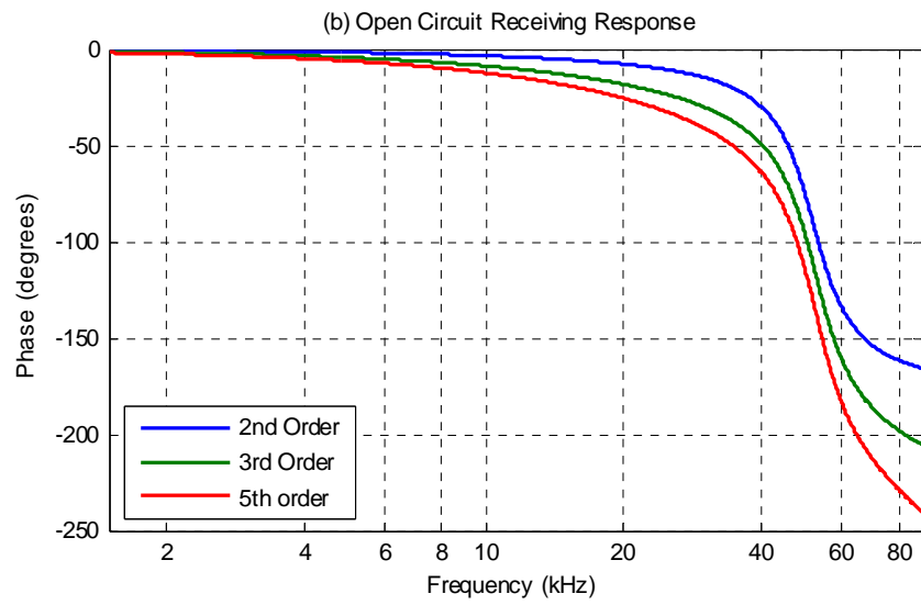
Figure 4.5 Simulated phase response of Rona hydrophone.
