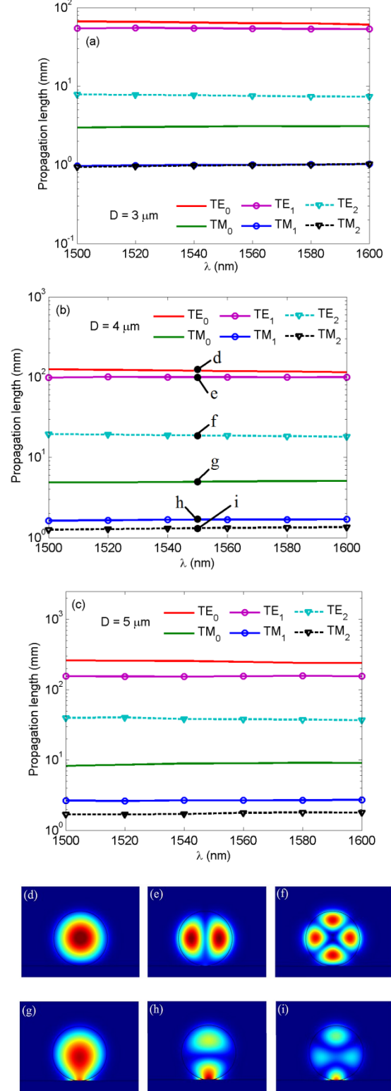
Fig.2 (a-c) Wavelength dependence of the propagation length for the microfiber with different diameter D for the TM and TE modes. Normalized electric energy distributions with D = 4 \mu\text{m} at the wavelength of 1550 nm: (d) \text{TE}_0 mode, (e) \text{TE}_1 mode, (f) \text{TE}_2 mode, (g) \text{TM}_0 mode, (h) \text{TM}_1 mode and (i) \text{TM}_2 mode.
