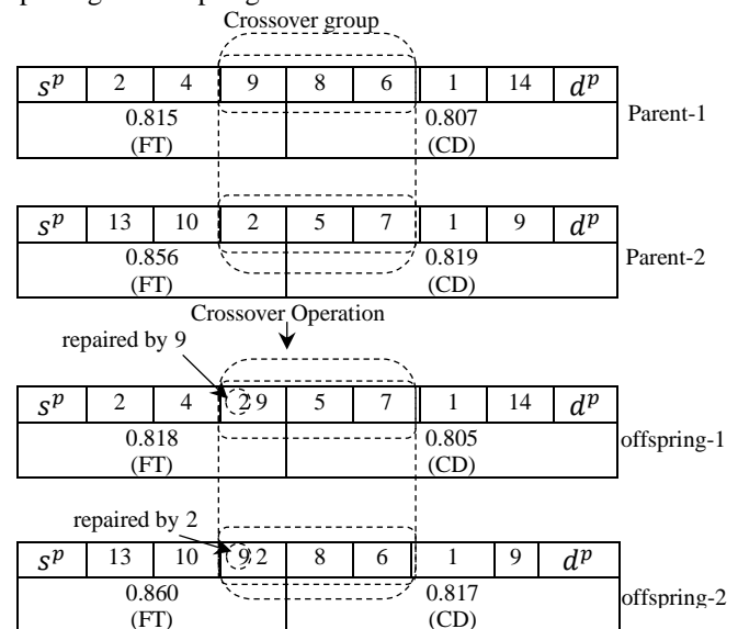
Fig. 4. The crossover operation
