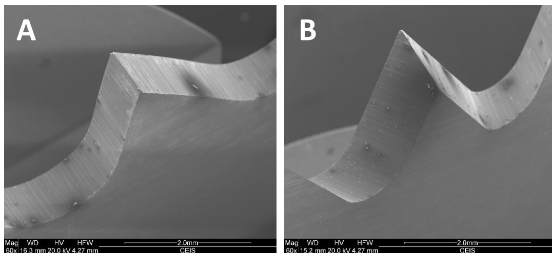
Figure 1: Micrograph images of the unbevelled handsaw tooth (A); and the bevelled handsaw tooth (B)
