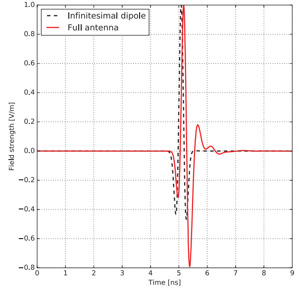
Fig. 5. Time domain responses (normalised) from the H-plane of an infinitesimal dipole model and the full antenna model at a distance of 0.58 m and an angle of 153^\circ in a lossless dielectric environment of relative permittivity \epsilon_r = 5 .
