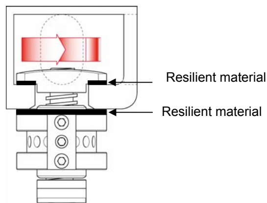
Figure 4: Detail of the initial design of the connector
