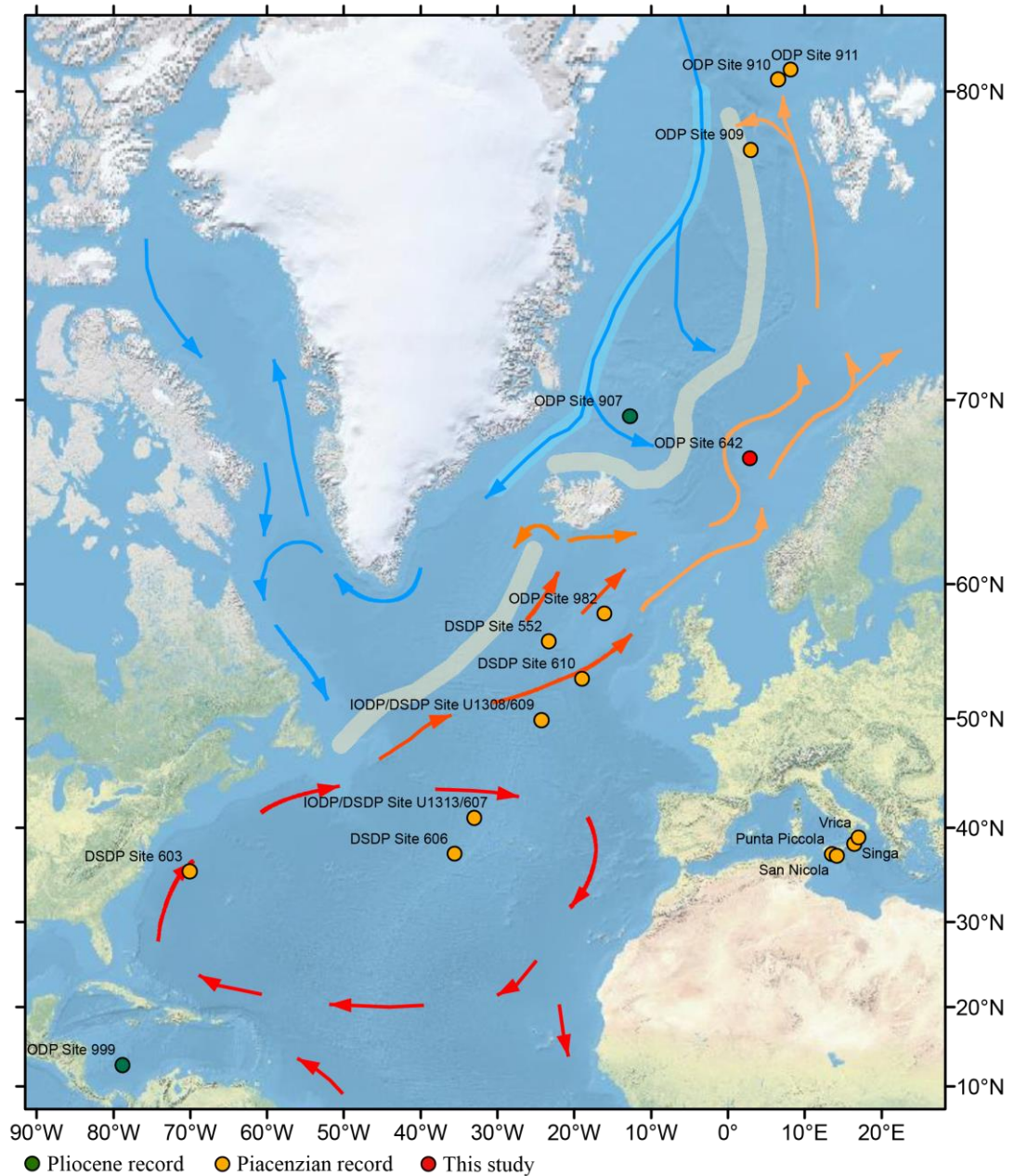
Figure 1.9: Location of Pliocene sea surface temperature records discussed in the text and modern-day ocean surface circulation in the North Atlantic and Nordic Seas. Colour coding is indicative of the relative temperature of the surface water masses: red = very warm; dark orange = warm; light orange = moderately warm; blue = cold. SSTs. SSTs decrease by 4.5°C between 3.5 and 2.5 Ma, supporting the notion that the onset of NHG was gradual and possibly reflecting the growth of a modern-like Greenland ice sheet. During the Piacenzian, SST changes led the benthic \delta^{18}\text{O} signal, indicating a larger contribution of ice volume as opposed to temperature to the \delta^{18}\text{O} signal (Lawrence et al., 2009). Sea surface temperatures for the mPWP were derived from multiple proxies at four sites in the mid-latitudes of the North Atlantic to evaluate potential biases with regard to the recorded environmental signal (e.g. spring/summer or
