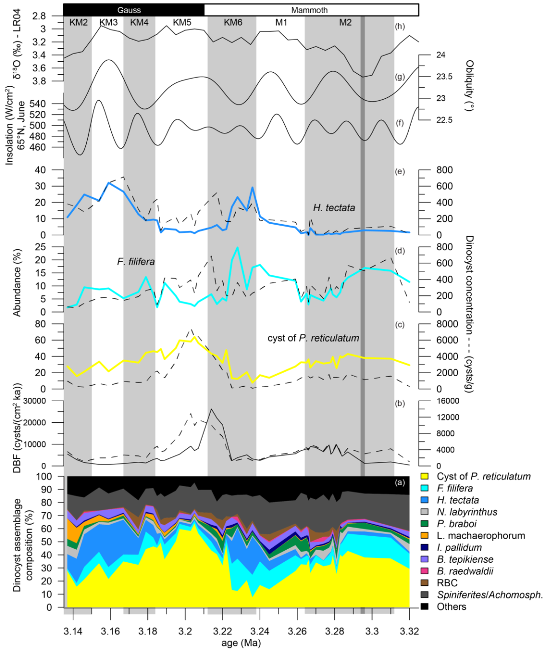
Figure 5.1: Abundances changes of selected dinoflagellate cyst (dinocyst) species from ODP Hole 642B (a–e) and orbital solutions for mean daily insolation (f) and obliquity (g) from Laskar et al. (2004) as well as the global benthic oxygen isotope stack (h) from Lisiecki and Raymo (2005). (a) Dinocyst assemblage composition in Hole 642B. cyst of P. reticulatum = Protoceratium reticulatum , F. filifera = Filisphaera filifera , H. tectata = Habibacysta tectata , N. labyrinthus = Nematosphaeropsis labyrinthus , P. braboi = Pyxidiniopsis braboi , L. machaerophorum = Lingulodinium machaerophorum , I. pallidum = Impagidinium pallidum , B. tepikiense = Bitectatodinium tepikiense , B. raedwaldii = Bitectatodinium raedwaldii , RBC = round brown cysts and Spinisph./Achomosphaera spp.; (b) dinocyst burial flux (DBF) and total dinocyst concentration and (c–e) relative abundance and concentration of the dinocyst species cyst of P. reticulatum , F. filifera and H. tectata . Dark grey vertical bar indicates the possible presence of an hiatus over the most extreme part of marine isotope stage M2 (Risebrobakken et al., 2016).
