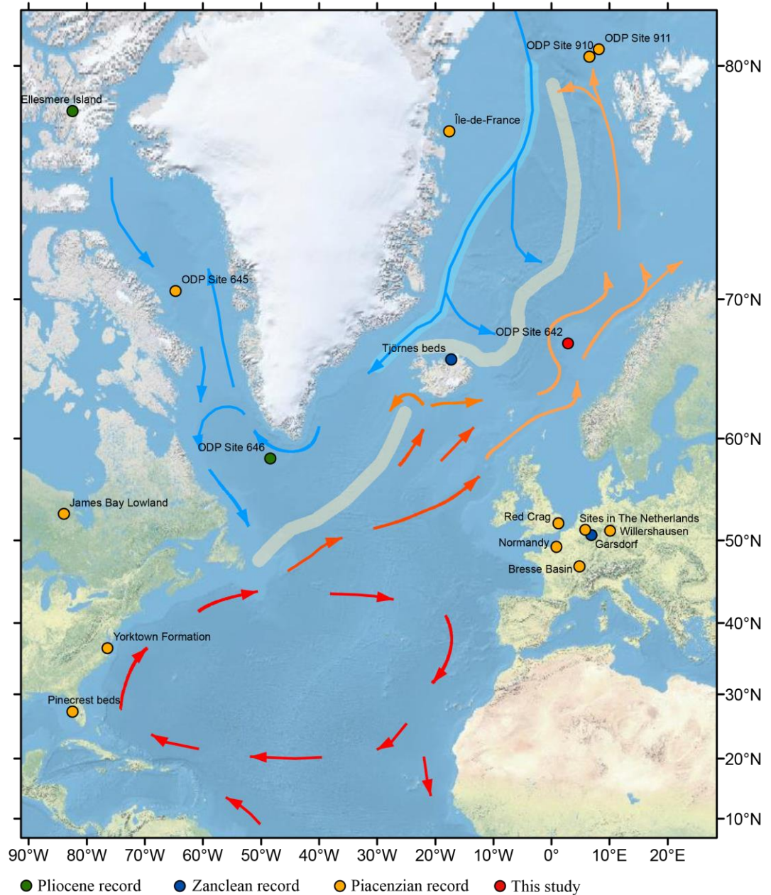
Figure 1.6: Location of Pliocene vegetation records discussed in the text and modern-day ocean surface circulation in the North Atlantic and Nordic Seas. Colour coding is indicative of the relative temperature of the surface water masses: red = very warm; dark orange = warm; light orange = moderately warm; blue = cold.
