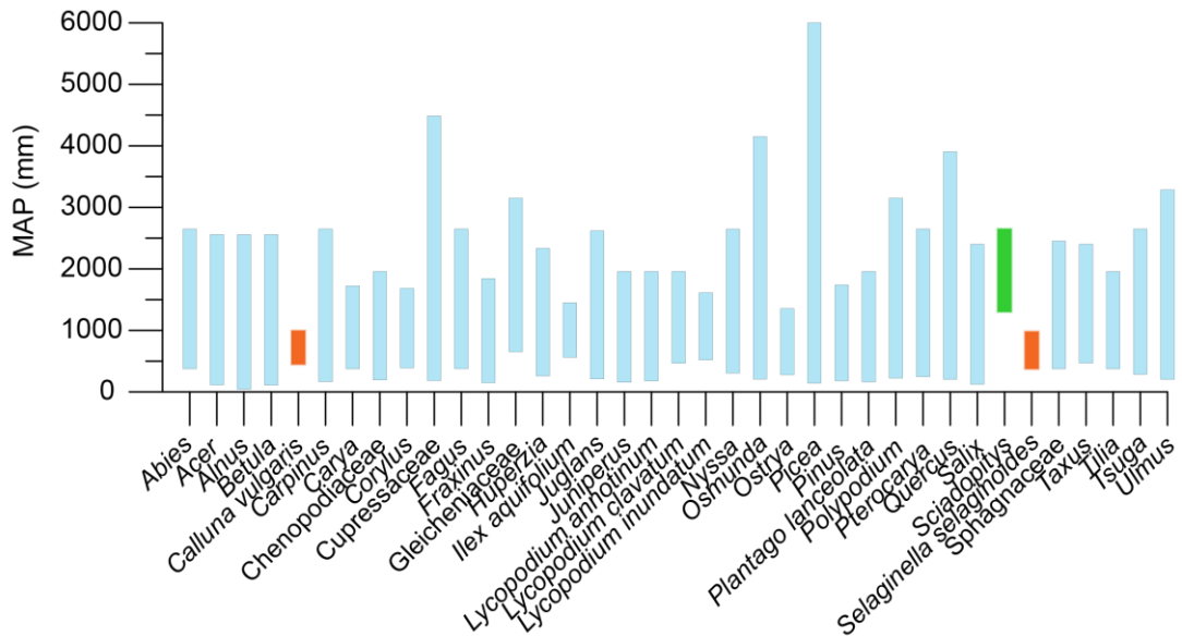
Figure 3.5: Mean annual precipitation (MAP) tolerances for taxa encountered in the Piacenzian samples from ODP Hole 642B. Green and orange bars show taxa that become climatic outliers if present in the same sample, producing two ambiguous coexistence intervals (Figure 3.4).
