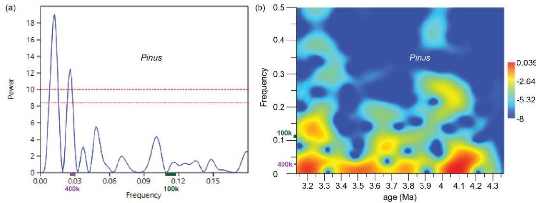
Figure 4.4: Spectral analysis of the relative abundance changes of (a) Pinus interpolated to 11,000 years and the corresponding evolutionary spectra (b). (a) Red dashed lines represent the 99% and 95% significance levels. (b) A size 32 Hanning window was used. The colours are indicative of the relative power. The purple and green bars along the frequency axes of both figures mark the frequency ranges of the 400,000-years and 100,000-years eccentricity cycles (data obtained from Laskar et al., 2004).
