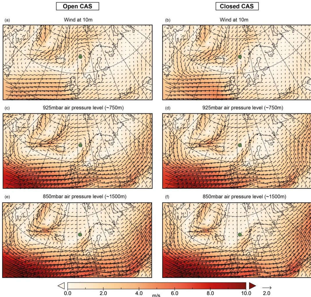
Figure 4.5: Model predictions for winds in spring (March, April, May) in the Nordic Seas region with an open and closed Central American Seaway (CAS). (a–b) winds at 10m altitude; (c–d) winds on the 925mbar pressure level, corresponding to an altitude of ~750m; and (e–f) winds on the 850mbar pressure level, corresponding to an altitude of ~1500m. The green circle marks the location of ODP Hole 642B in the Norwegian Sea (67°N, 3°E).
