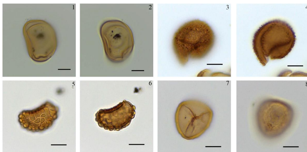
Plate 3.4: Selected pollen species from ODP Hole 642B. All images were taken in bright field illumination. Sample number and England Finder coordinates are given after species name. Scale bar represents 10 \mu\text{m} . 1–8: Spores of ferns and mosses, 1–2: psilate monolete undifferentiated, 9H2 15-16, O41/1; 3–4: Osmunda , 9H2 130-131, Q49/0; 5–6: Polypodium , 9H2 130-131, S37/2; 9–10: Sphagnum , 9H2 75-76, R40/0.
