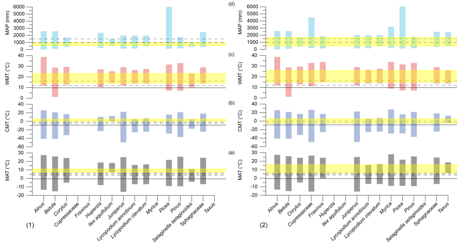
Figure 3.6: Climatic tolerances of taxa found in the (1) modern sample (0 cm) and (2) mid-Holocene sample (3cm) for (a) mean annual temperatures (MAT), (b) coldest month temperatures (CMT), (c) warmest month temperatures (WMT) and (d) mean annual precipitation (MAP). Yellow bars show the coexistence intervals for each parameter. Solid black lines in panels (a) to (c) represent the modern climate values from the meteorological stations in Bodø and Mo i Rana, Nordland, Norway ( Figure 2.1 ) (Norwegian Meteorological Institute and Norwegian Broadcasting Corporation, 2014). Dashed lines represent the range of modern coastal temperatures (Moen, 1999). Listed taxa are found in both the modern and mid-Holocene samples.
