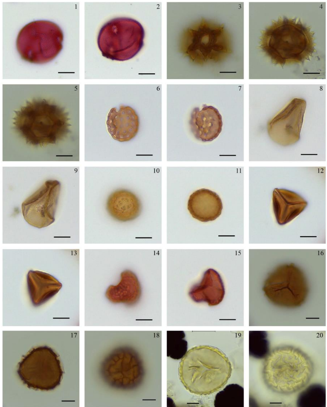
Plate 3.3: Selected pollen species from ODP Hole 642B. All images were taken in bright field illumination. Sample number and England Finder coordinates are given after species name. Scale bar represents 10 \mu\text{m} . 1–2: Pollen of deciduous trees, 3–11: pollen of herbs, 12–20: spores ferns and mosses. 1–2: Tilia , 9H7 61-62, M37/2; 3–5: Asteraceae Liguliflorae type, 9H2 90-91, K56/2; 6–7: Chenopodiaceae, 9H2 130-131, V49/3; 8–9: Cyperaceae, 10H1 45-46, N52/1; 12–13: Gleicheniaceae, 9H2 135-136, V38/1; 14–15: Huperzia , 9H3 25-26, R40/4; 16–18: Lycopodium annotinum , 9H2 15-16, F62/3; 19–20: Lycopodium inundatum , 10H4 115-116, W40/0.
