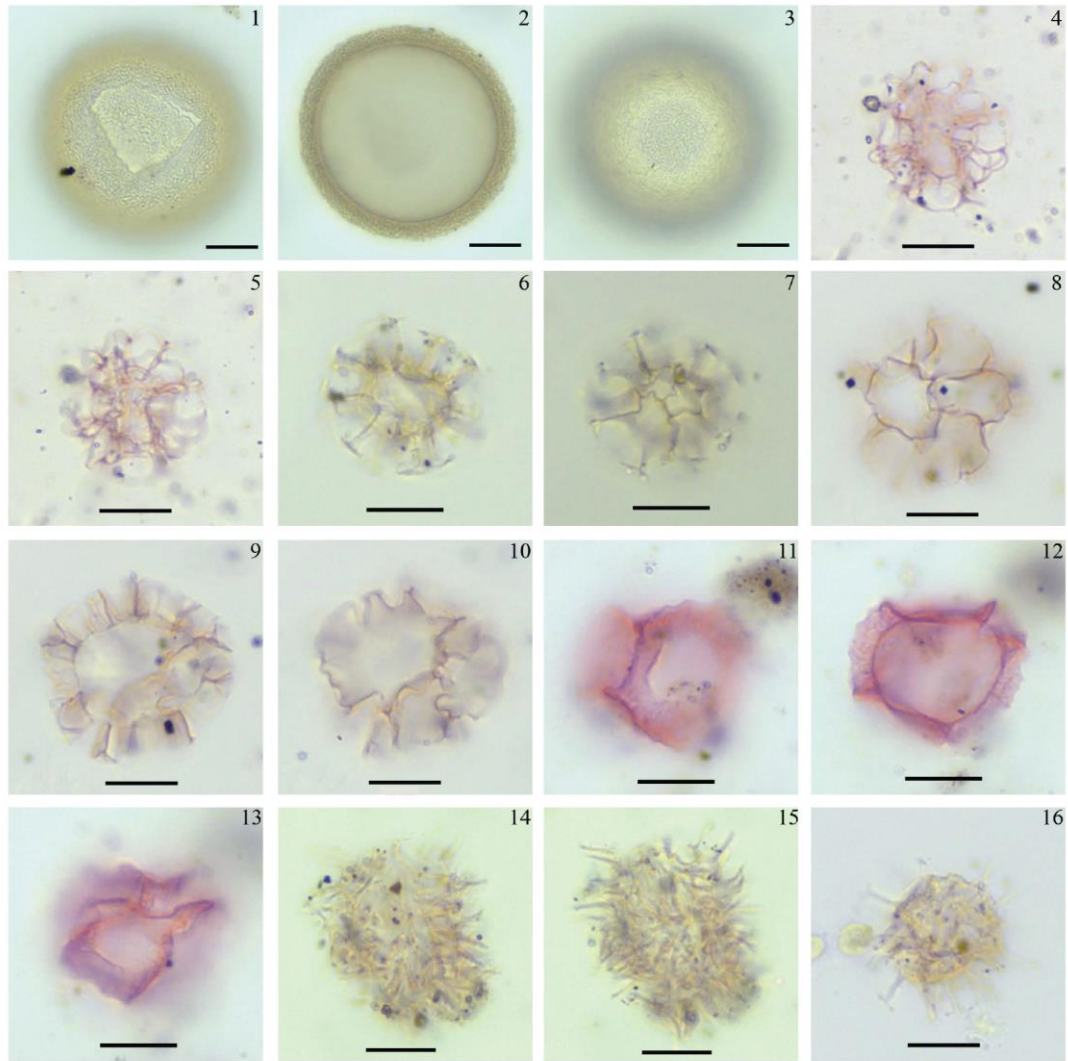
Plate 5.4: Selected dinoflagellate cysts and acritarch species from ODP Hole 642B. All images were taken in bright field illumination. Sample number and England Finder coordinates are given after species name. Scale bar represents 10 \mu m. 1-3: Tectatodinium pellitum , 9H1 76-77, J35/4; 4-5: Cymatiosphaera? aegirii , 9H1 67-86, N38/0; 6-7: Cymatiosphaera? icenorum , 9H2 34-35, K36/0; 8-10: Cymatiosphaera? invaginata , 9H1 115-116, W36/2; 11-13: Lavradospaera crista , 9H1 90-91, O49/0; 14-15: Nannobarbophora walldalei , 9H2 48-49, M35/0; 16: Small spiny acritarch, 9H2 30-31, F42/0.
