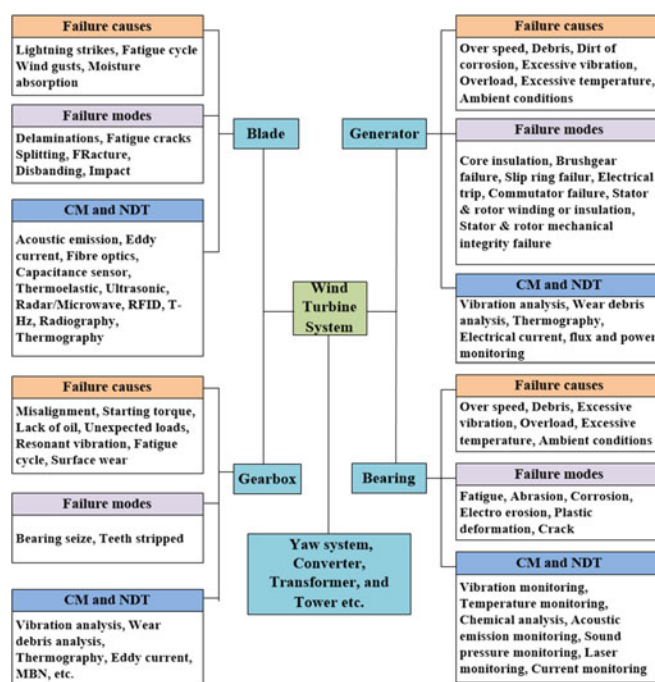
Fig. 2. Failure causes, modes and relevant CM and NDT methods for major components in wind turbine systems.
