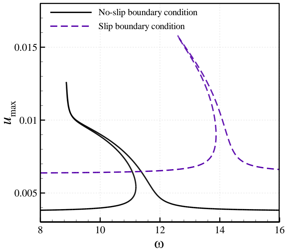
Fig. 14. Effects of slip boundary conditions on the forced oscillation when U=6.4 (supercritical flow regime); (a) w_{\max} at x=0.5 ; (b) u_{\max} at x=0.657 .
