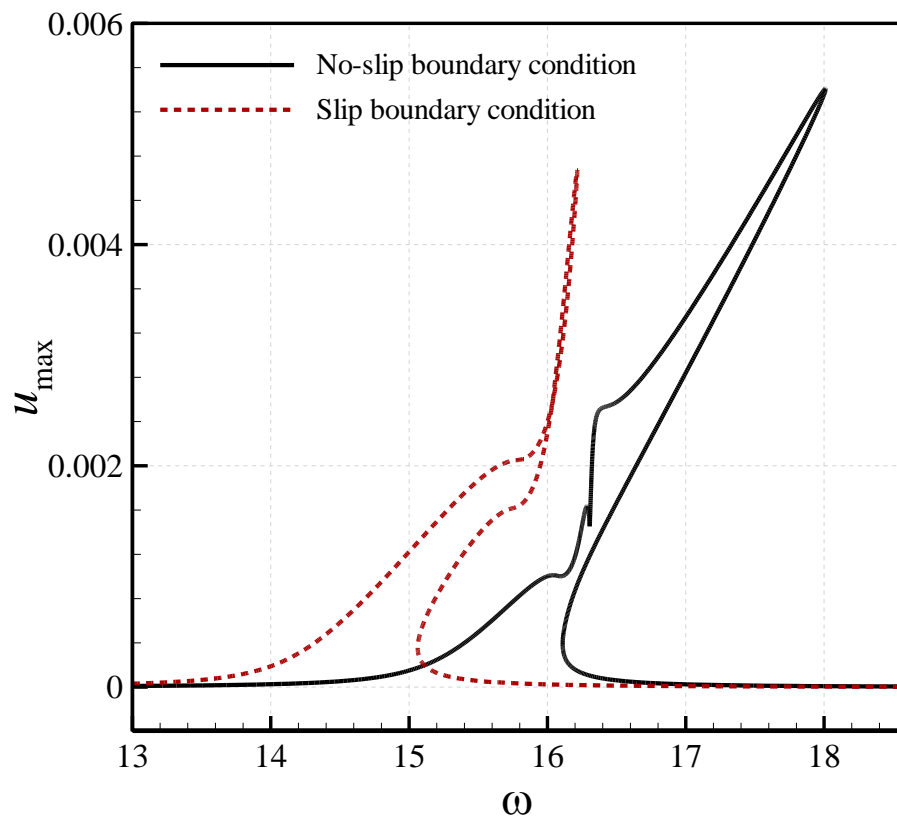
Fig. 7. Effects of slip boundary conditions on the forced oscillation when U=3.5 (subcritical flow regime); (a) w_{\max} at x=0.5 ; (b) u_{\max} at x=0.657 .
