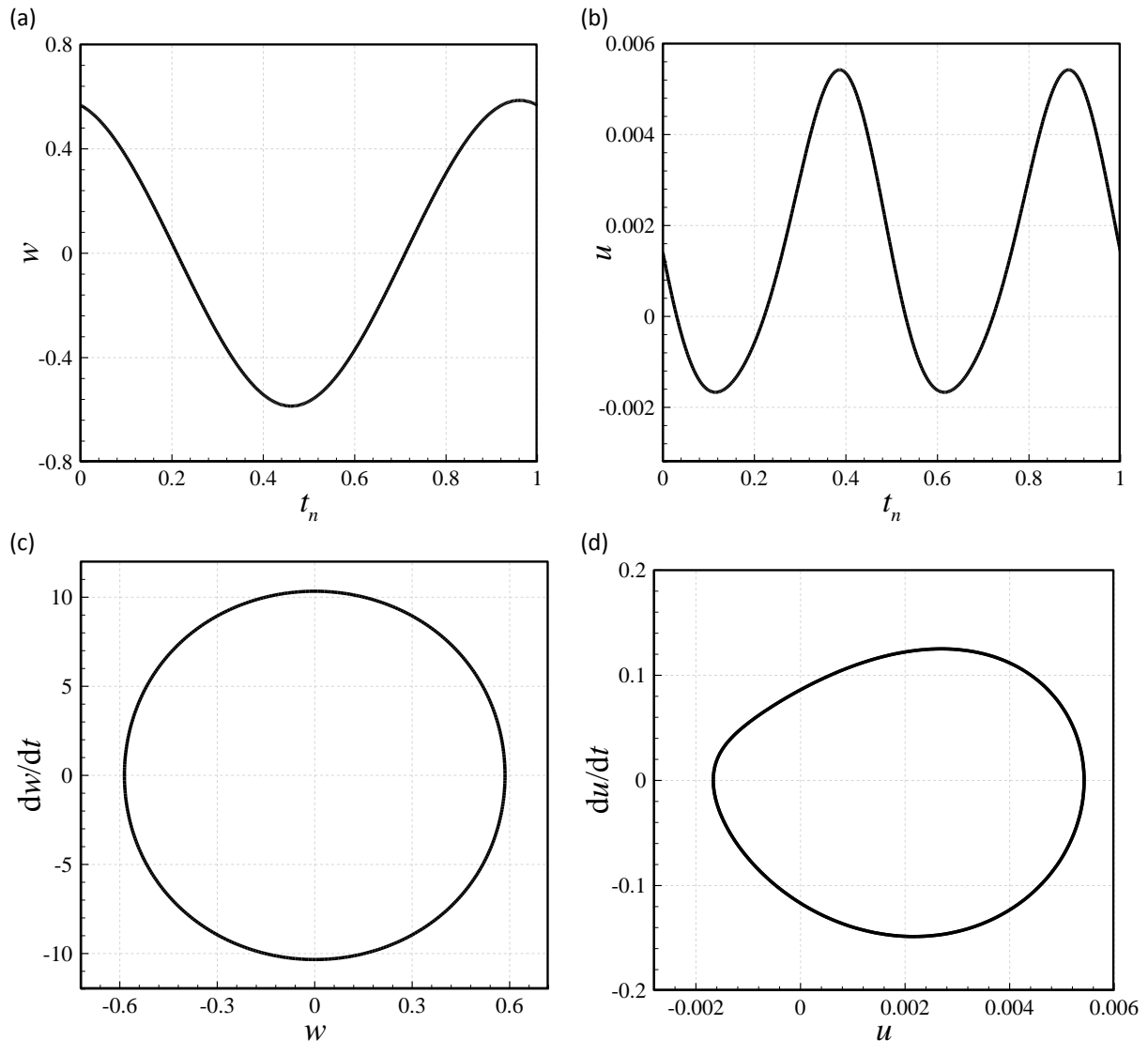
Fig. 5. Detailed motion characteristics of the system of Fig. 2 at \omega/\omega_1=1.1608 (i.e. at peak oscillation amplitude). (a, b) w versus t_n for x=0.5 and u versus t_n for x=0.657 , respectively; (c, d) dw/dt versus w for x=0.5 and du/dt versus u for x=0.657 , respectively.
