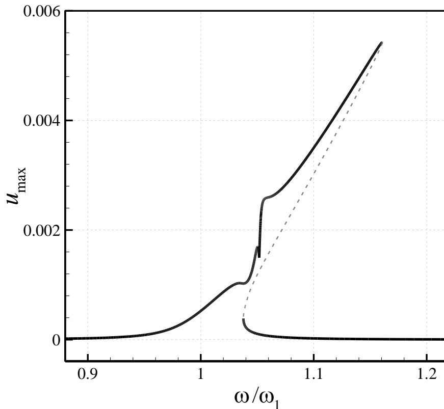
Fig. 2. Change of maximum transverse and axial displacements versus the frequency ratio in the subcritical flow regime for F_1=2.0 and U=3.25 ; (a) w_{\max} at x=0.5 ; (b) u_{\max} at x=0.657 ; \omega_1=15.5031 .
