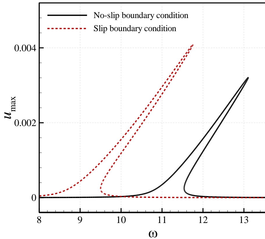
Fig. 8. Effects of slip boundary conditions on the forced oscillation when U=4.5 (subcritical flow regime); (a) w_{\max} at x=0.5 ; (b) u_{\max} at x=0.657 .
