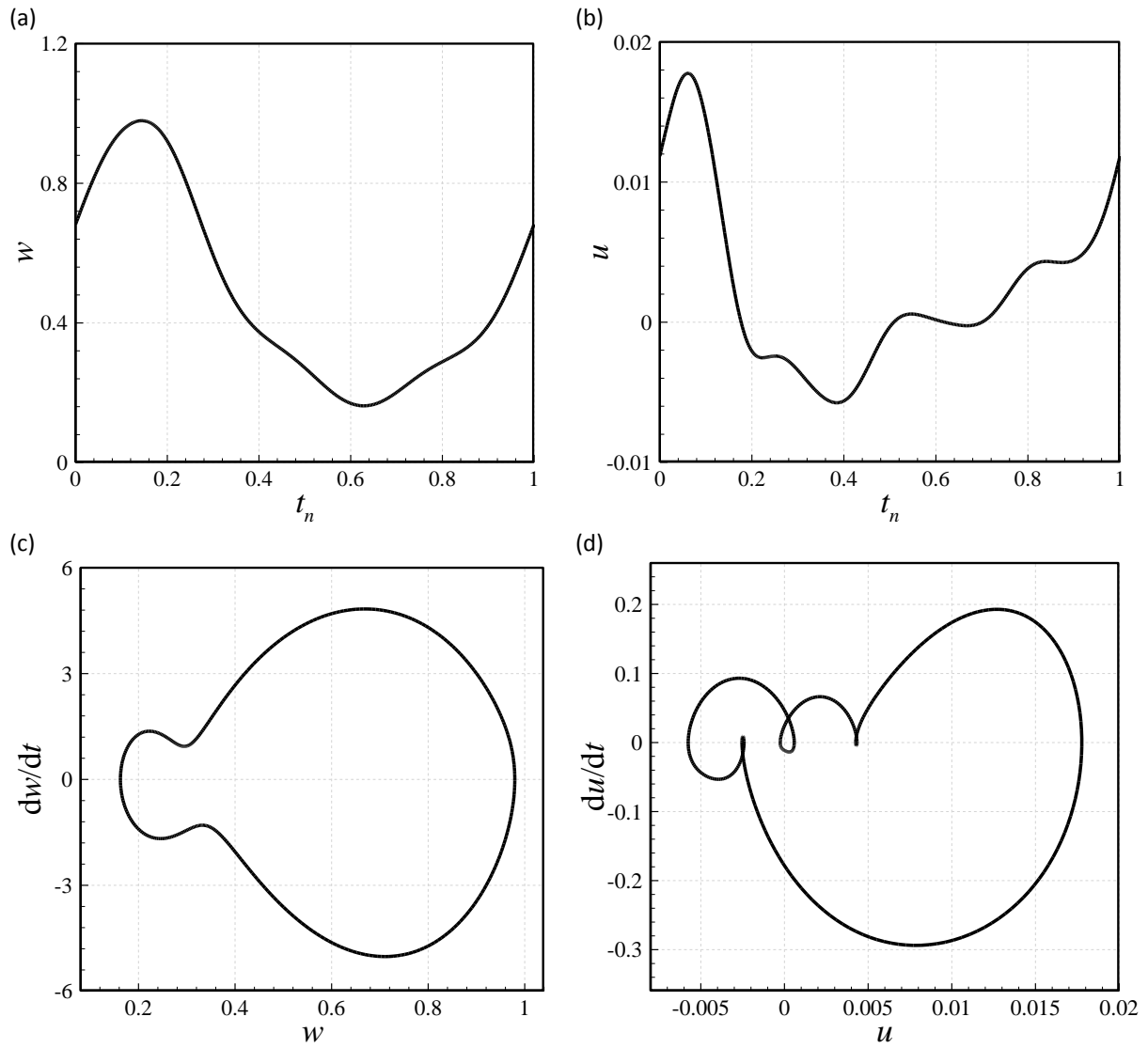
Fig. 12. Detailed motion characteristics of the nanosystem of Fig. 10 at \omega/\omega_1=0.6705 . (a, b) w versus t_n for x=0.5 and u versus t_n for x=0.657 , respectively; (c, d) dw/dt versus w for x=0.5 and du/dt versus u for x=0.657 , respectively.
