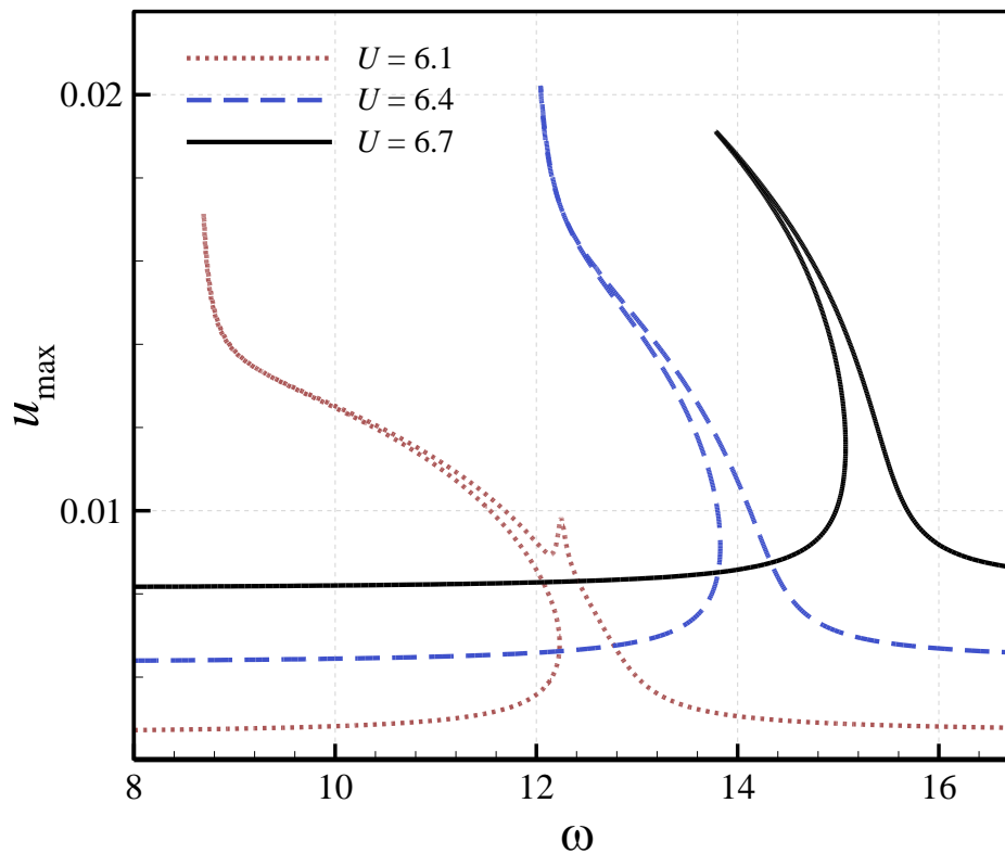
Fig. 13. Change of maximum transverse and axial displacements versus the excitation frequency for different fluid speeds in supercritical flow regime; (a) w_{\max} at x=0.5 ; (b) u_{\max} at x=0.657 .
