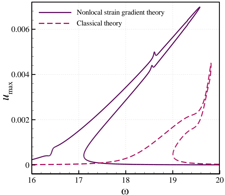
Fig. 9. Change of maximum transverse and axial displacements versus the excitation frequency obtained via the nonlocal strain gradient theory and classical theory for U=3.0 (subcritical flow regime); (a) w_{\max} at x=0.5 ; (b) u_{\max} at x=0.657 .
