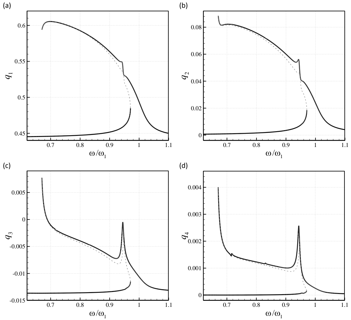
Fig. 11. Change of (a) q_1 , (b) q_2 , (c) q_3 and (d) q_4 versus the ratio of the excitation frequency to the natural one in the supercritical flow regime.
