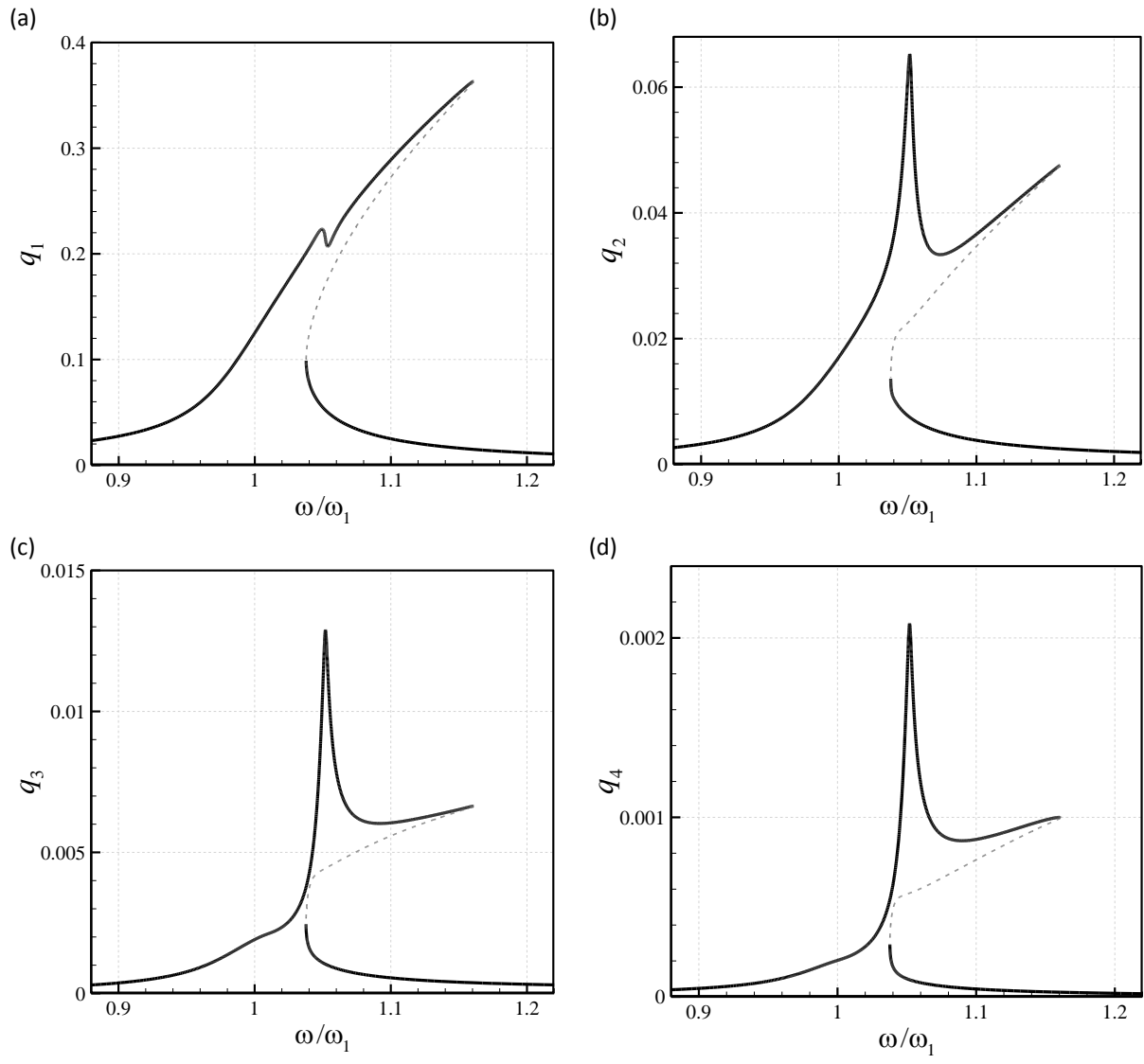
Fig. 3. Change of (a) q_1 , (b) q_2 , (c) q_3 and (d) q_4 versus the ratio of the excitation frequency to the natural one in the subcritical flow regime.
