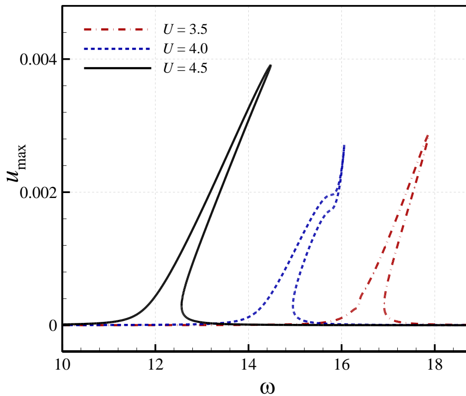
Fig. 6. Change of maximum transverse and axial displacements versus the excitation frequency for different fluid speeds in subcritical flow regime; (a) w_{\max} at x=0.5 ; (b) u_{\max} at x=0.657 .
