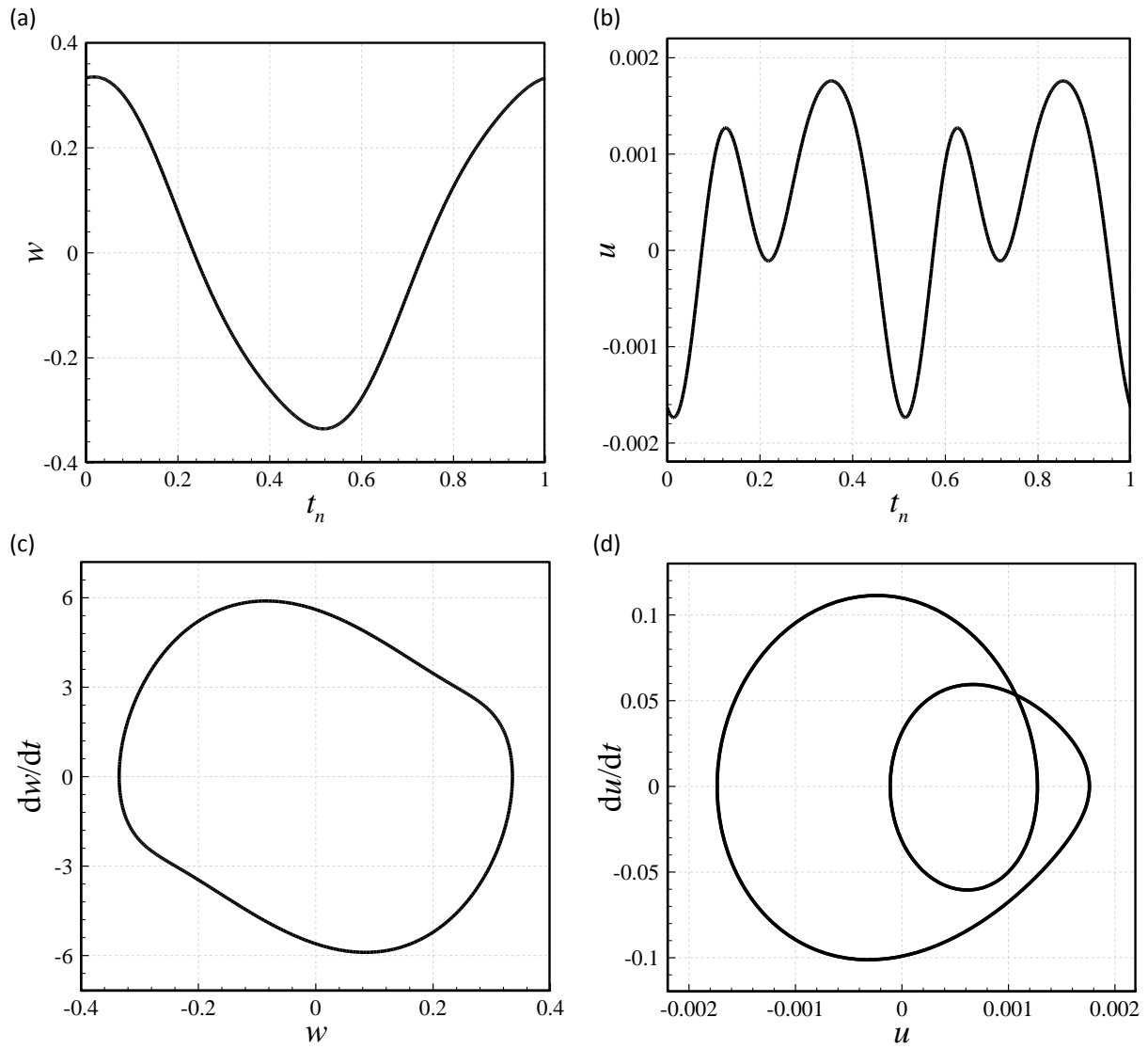
Fig. 4. Detailed motion characteristics of the system of Fig. 2 at \omega/\omega_1=1.0522 (i.e. when the modal interactions are strongest). (a, b) w versus t_n for x=0.5 and u versus t_n for x=0.657 , respectively; (c, d) dw/dt versus w for x=0.5 and du/dt versus u for x=0.657 , respectively.
