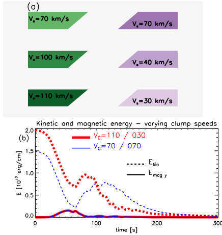
Fig. 10. Panel a : sketch of some simulations of the parameter space investigation where the speeds between the clumps are varied. Panel b : evolution of the kinetic and magnetic energy for the simulations where the clump speeds are both 70 \text{ km s}^{-1} and where they are 110 \text{ km s}^{-1} and 30 \text{ km s}^{-1} .
