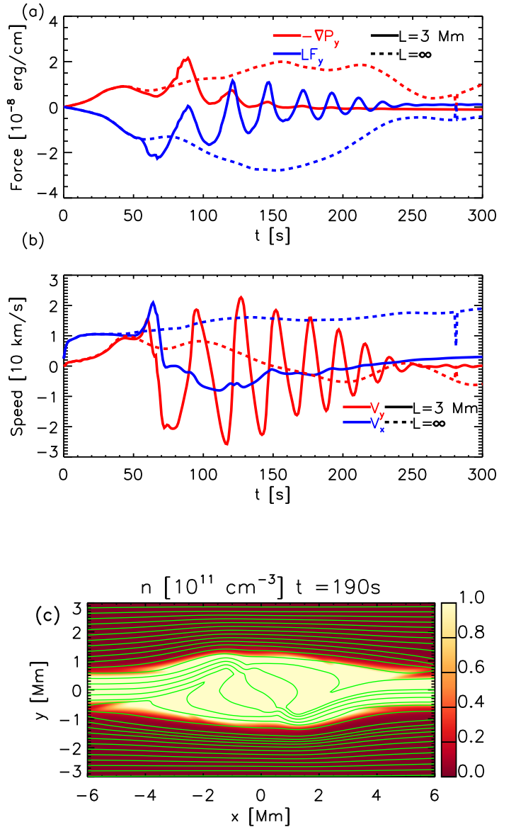
Fig. 18. Panel a: evolution of the y-axis components of the gas pressure gradient and Lorentz force averaged over the rectangular region shown in Fig. 2 for the simulations with clump length L = 3 Mm and infinite. Panel b: evolution of the x- and y-axis components of the velocity averaged over the rectangular region shown in Fig. 2 for the simulations with clump length L = 3 Mm and infinite. Panel c: map of the number density n at t = 190 s for the simulation with infinite clump length. Green lines are magnetic field lines drawn from the left-hand boundary.
