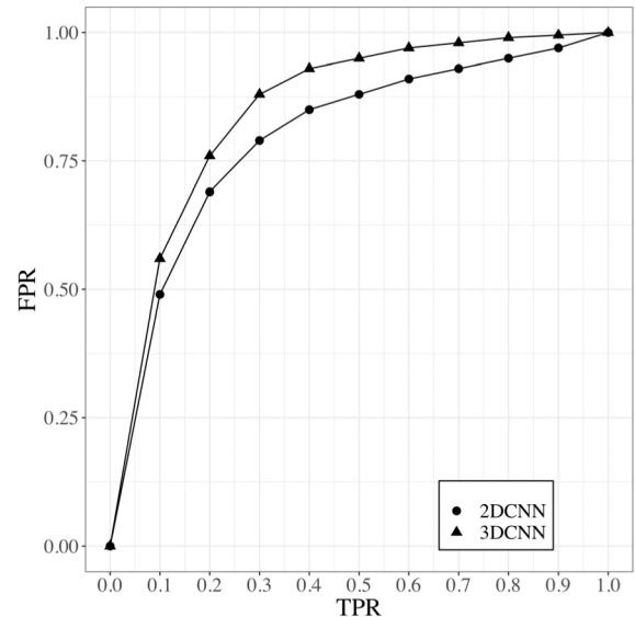
FIGURE 10. The Classification Results of Enhanced rate image ROI and VOI.
