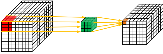
FIGURE 2. Three-dimensional convolutional neural network (3DCNN).
