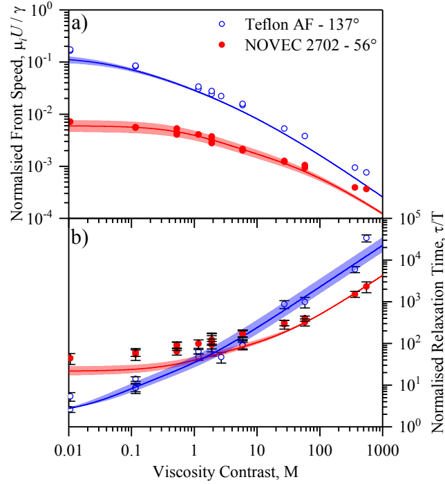
Figure 3. Linear and exponential dewetting regimes. a) Speed of the dewetting front, U , vs viscosity ratio, M , during the linear dewetting regime of the thin film. The speed is normalized using the characteristic speed \gamma/\mu_i , where \gamma is the interfacial tension and \mu_i is the viscosity of the (inner) dewetting liquid. b) Exponential time constant, \tau , vs viscosity ratio, M , during the exponential relaxation of the droplet towards equilibrium. The relaxation time is normalized using the characteristic time T = \mu_i \Omega^{1/3} / \gamma , where \Omega is the droplet volume. The blue (empty) and red (full) symbols correspond to experimental results on Teflon and NOVEC surfaces, respectively. The solid lines correspond to the theoretical prediction of equations 4 and 8, using an inner fluid viscosity \mu_i = 189 \text{ mPa s} , interfacial tension \gamma = 6.2 \text{ mN m}^{-1} , rim radius R_f = 1 \text{ mm} and film thickness h_0 = 50 \text{ }\mu\text{m} , all set using the experimentally measured values. The light-colored bands correspond to the uncertainty in the theoretical prediction due to the uncertainty in the equilibrium contact angle. Error bars for M and \mu_i U / \gamma are smaller than the symbols; error bars for \tau / T correspond to the uncertainty in the fit to an exponential of the data of the instantaneous base radius of the dewetting liquid, R , vs time, t .
