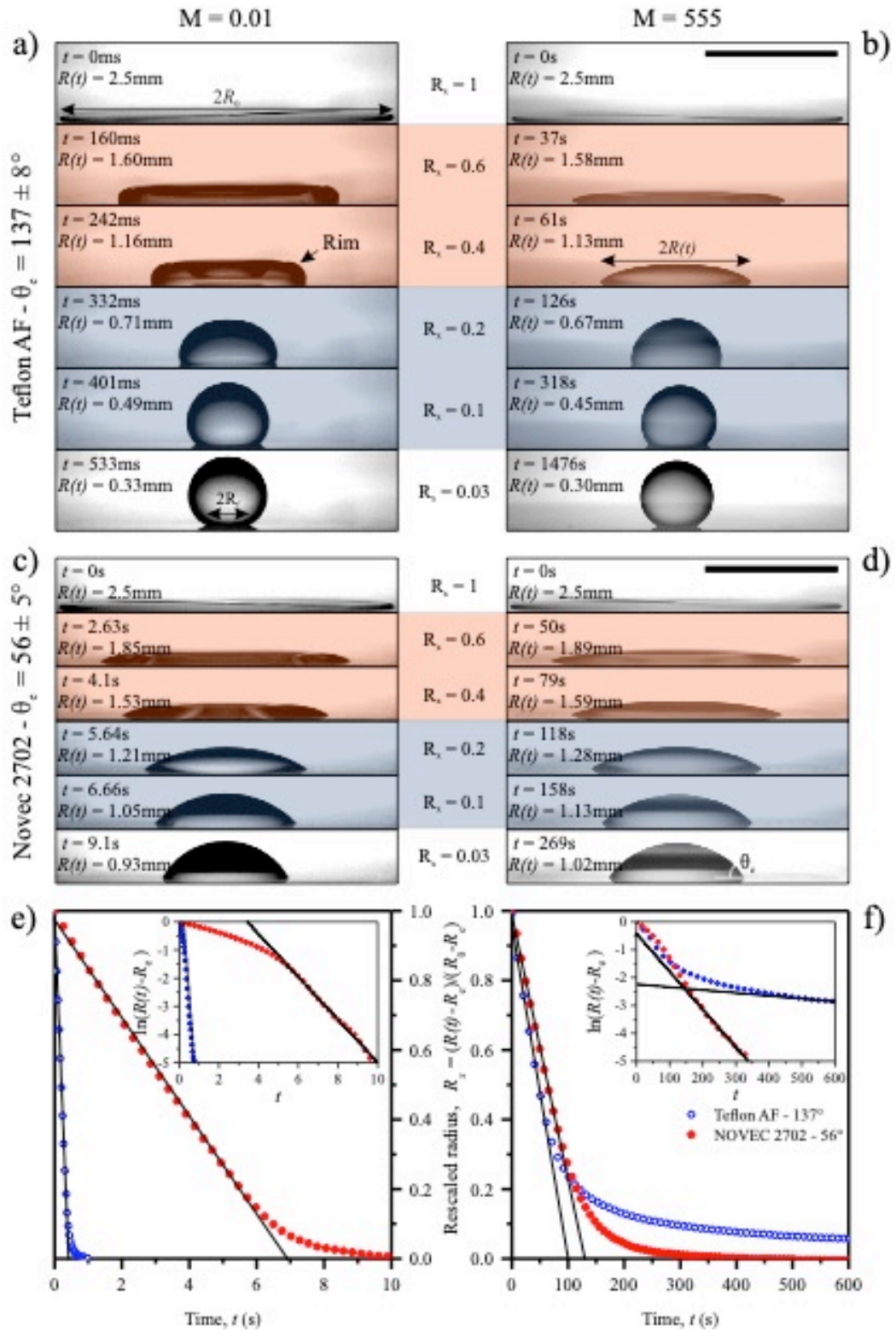
Figure 1. Liquid-liquid film dewetting. a) and b): Time-sequence images of the dewetting of a trimethylolpropane triglycidyl ether (TMP-TG-E) film on a Teflon surface (high film repellency) at viscosity ratio a) M=0.01 and b) M=555 . c) and d): Time-sequence images of the dewetting of a TMP-TPG-E film on a NOVEC 2702 surface (low film repellency) at c) M=0.01 and d) M=555 . e) and f): Rescaled radius R_x(t) vs time t for e) M=0.01 and f) M=555 for a single experiment on surfaces of different film repellency. The blue (empty) and red (full) symbols correspond to Teflon and NOVEC surfaces, respectively. The inset shows the exponential fitting to the data. The scale bars correspond to 2 mm.
