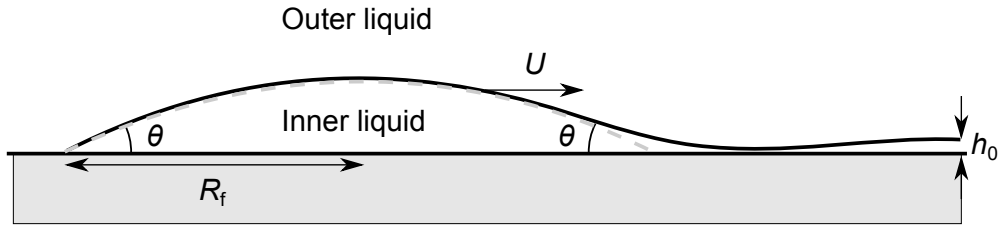
Figure 2. Schematic representation of a dewetting rim. The interface profile is approximated by a circular arc of base radius R_f and apparent contact angle \theta at the receding and the advancing edges. The rim connects to a film of typical thickness h_0 . The rim recedes at a speed U .
