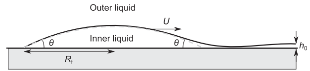
Fig. 2 Schematic representation of a dewetting rim. The interface profile is approximated by a circular arc of base radius R_f and apparent contact angle \theta at the receding and the advancing edges. The rim connects to a film of typical thickness h_0 . The rim recedes at a speed U .
