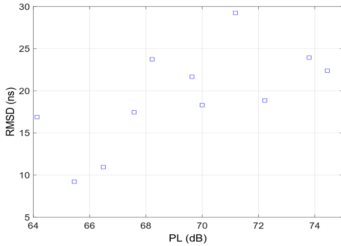
(b): RMSD variation with path loss at 28 GHz.
