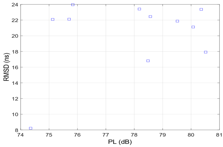
(c): RMSD variation with path loss at 38 GHz.
