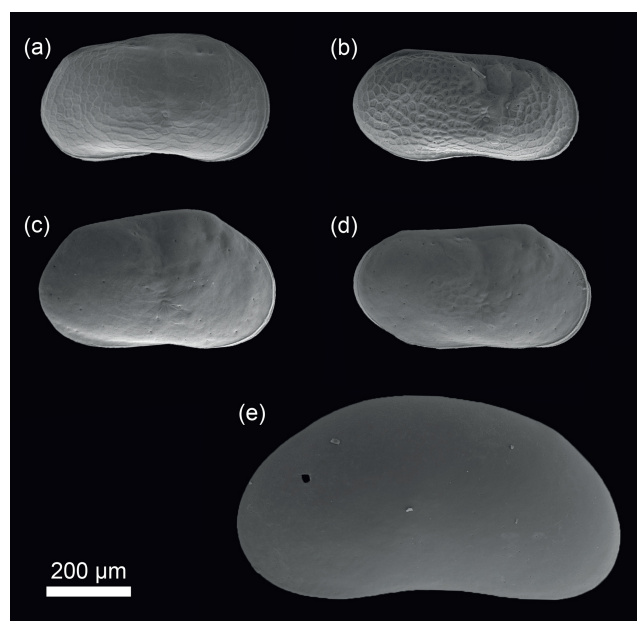
Figure 1. SEM photographs of the external lateral views of key species used in this study. (a) Female right valve Limnocythere inopinata , (b) male right valve Limnocythere inopinata , (c) female right valve Limnocythere sp. A, (d) male right valve Limnocythere sp. A and (e) female left valve Candona sp.
