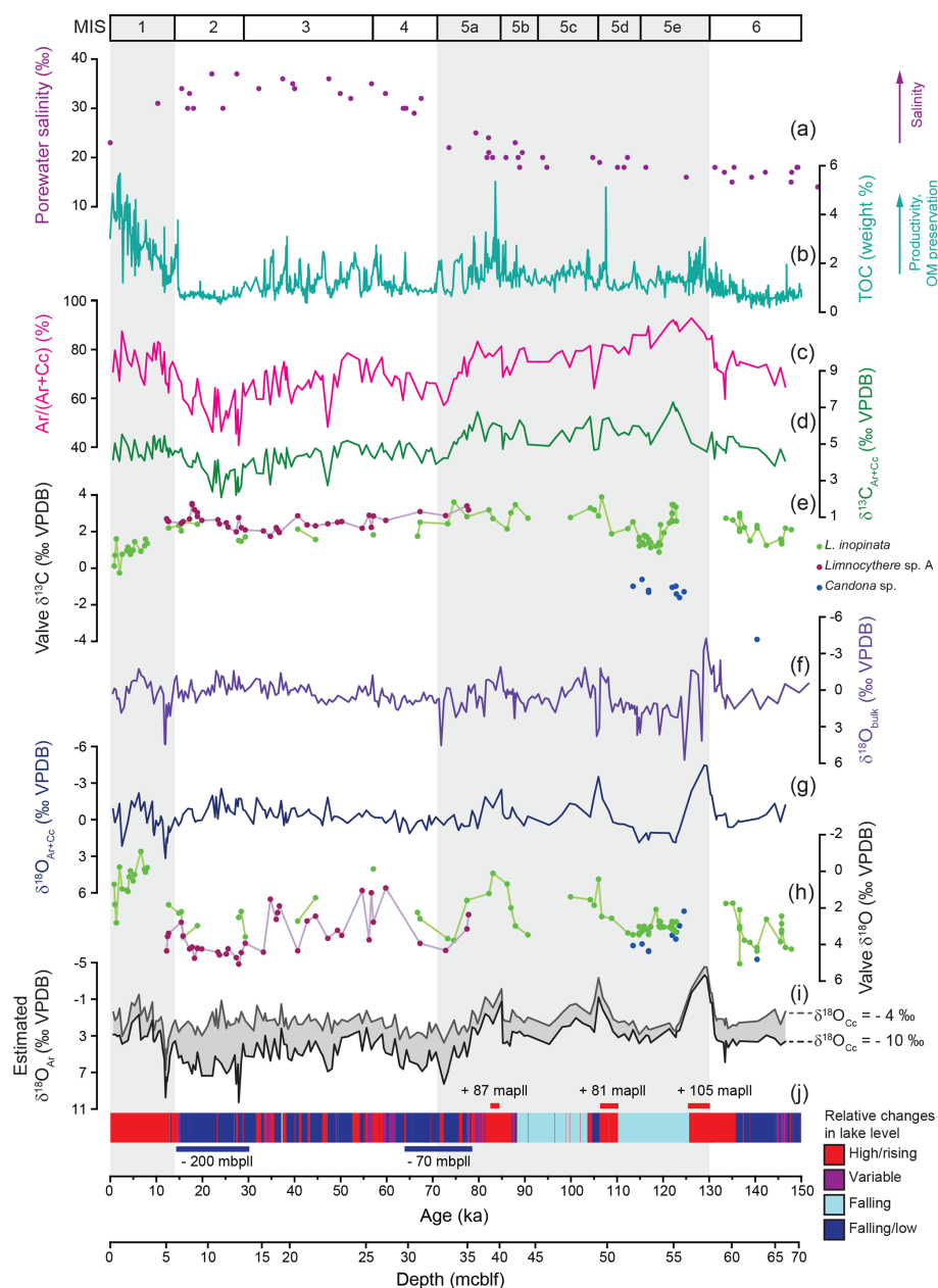
Figure 8. Ostracod isotopy compared with porewater salinity and inorganic carbonate isotopy and mineralogical composition. (a) Porewater salinity plotted against depth in metres' composite below lake floor (mcbf; Tomonaga et al., 2017). (b) Total organic carbon content (Stockhecke et al., 2014a). (c, d, g, i) Inorganic mineralogy and isotopy from McCormack et al. (2019). (c) Relative aragonite content of dolomite poor samples (< 15 % dolomite) expressed by an aragonite / non-dolomite ratio Ar / (Ar + Cc) in weight % and (d, g) isotopic composition of dolomite poor samples ( \delta^{13}C_{Ar+Cc} and \delta^{18}O_{Ar+Cc} ). (f) Bulk carbonate oxygen isotope composition from Kwiecien et al. (2014). (i) Estimated \delta^{18}O_{Ar} values for \delta^{18}O_{Cc} values between -4\text{‰} and -10\text{‰} . (j) Lithology-based relative lake level changes (simplified according to Stockhecke et al., 2014a) and major lake level variations (Stockhecke et al., 2014a; Tomonaga et al., 2017) in metres above/below present lake level (mapll/mbpll). (e, h) Valve \delta^{18}O values and \delta^{13}C values.
