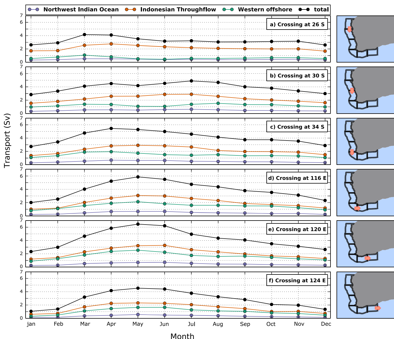
Figure 6. Mean seasonal contribution of Leeuwin Current sources along the Leeuwin Current's downstream flow, as located by the coral arrows in the maps on the right, for each row. Units are in Sv and the mean is taken over the years 1966–2003 and depth-integrating to 300 m. Orange lines are particles originating from the Indonesian Throughflow region, purple lines are from the northern offshore section, and green lines from the western offshore section. The black lines are the totals of the three colored lines.
