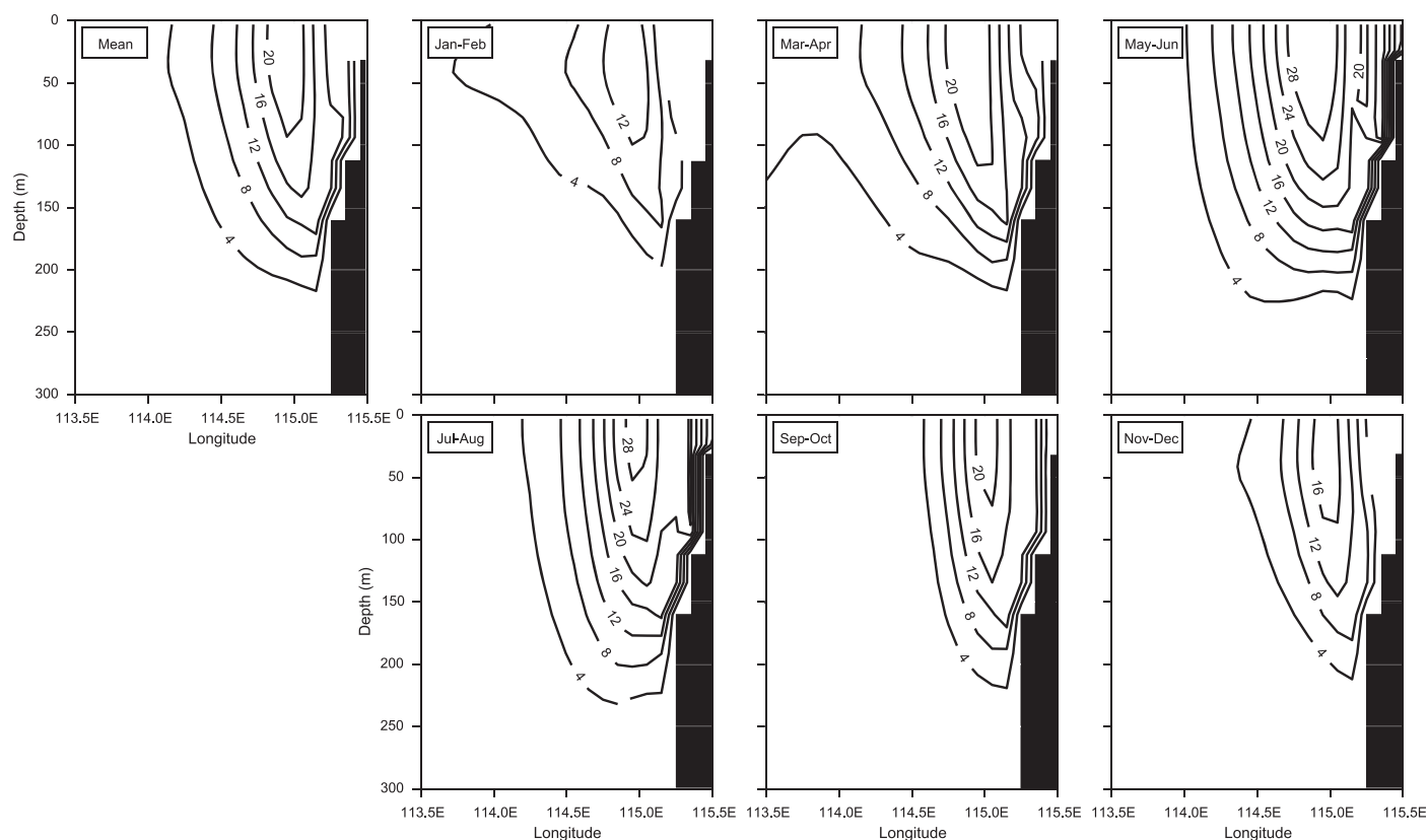
Figure 2. (top left) Mean and bimonthly mean (1960–2009) meridional velocity (m/s) at 32°S in the TROPAC01 model. Contours are 0.04 m/s and only negative velocities are shown.
