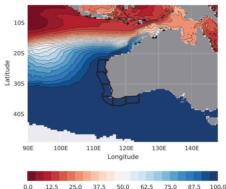
Figure 4. Connectivity map between the northern offshore/Indonesian Throughflow particles and the Leeuwin Current region as diagnosed from Lagrangian trajectories. The proportion of transport in each 0.5^\circ \times 0.5^\circ grid cell from trajectories that entered the Leeuwin Current region (blue) and trajectories that did not (red). A blue value above 50% indicates that the grid cell was dominated by trajectories that entered the Leeuwin Current region. The Leeuwin Current region is defined as any sectors pictured by the thick black lines. This figure demonstrates the importance of the Leeuwin Current as a pathway for water between the northern offshore region/Indonesian Throughflow and Australia's midlatitude and South Australian coastlines.
