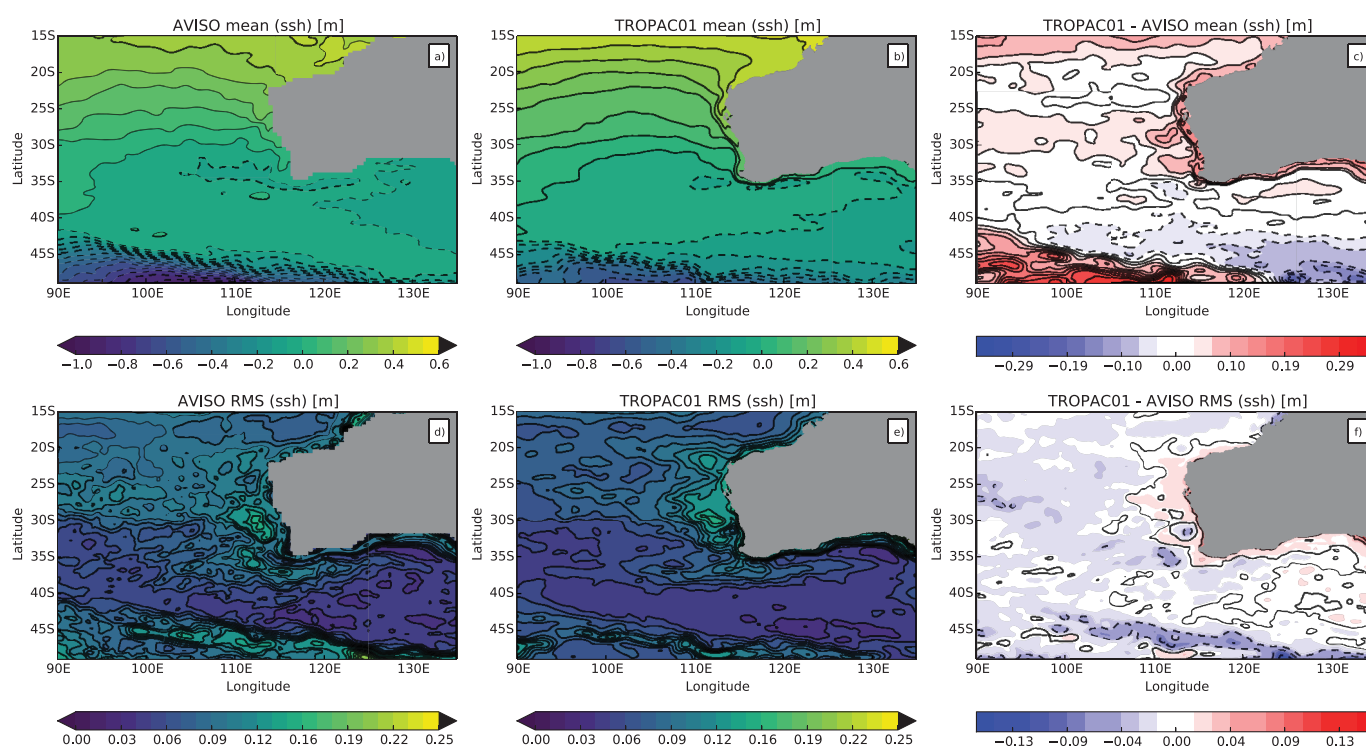
Figure 1. Evaluation of the TROPAC01 model: comparing the model sea surface height data for the period 1993–2009 to AVISO altimetry data over the same period. (a–c) Comparison of mean sea surface height. (d–f) Comparison of sea surface height variability, computed as the local root-mean-square variance of the sea surface height time series.
