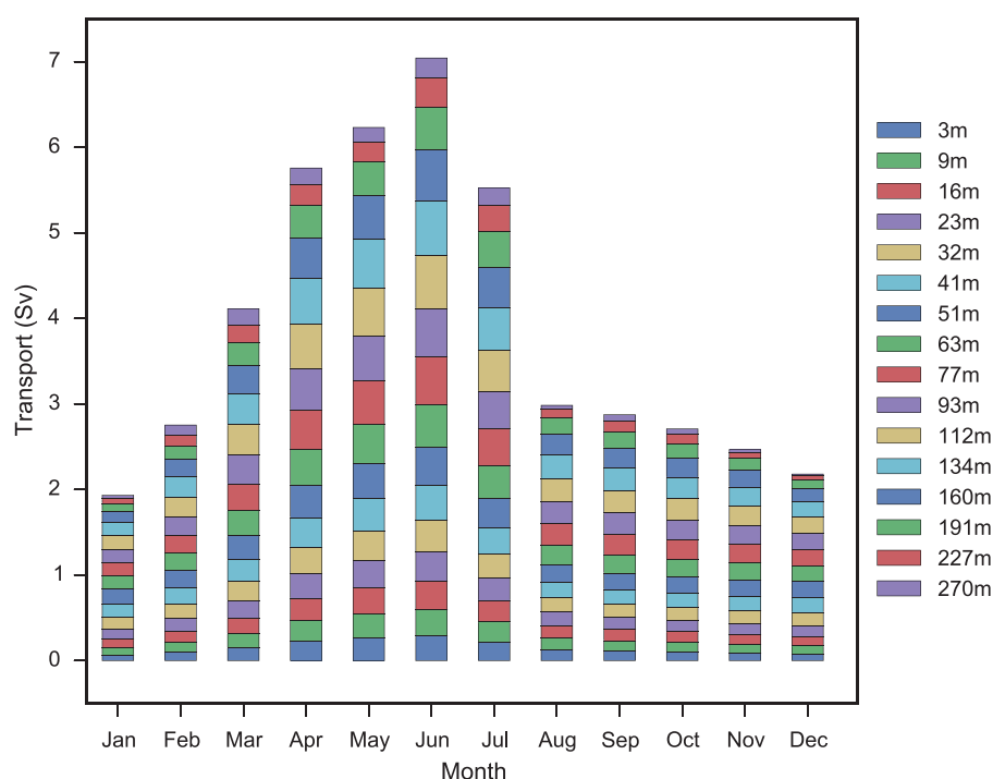
Figure 3. Eulerian southward transport from TROPAC01 at 32°S for years 1960–2009. Bar colors are different groupings of levels from TROPAC01.
