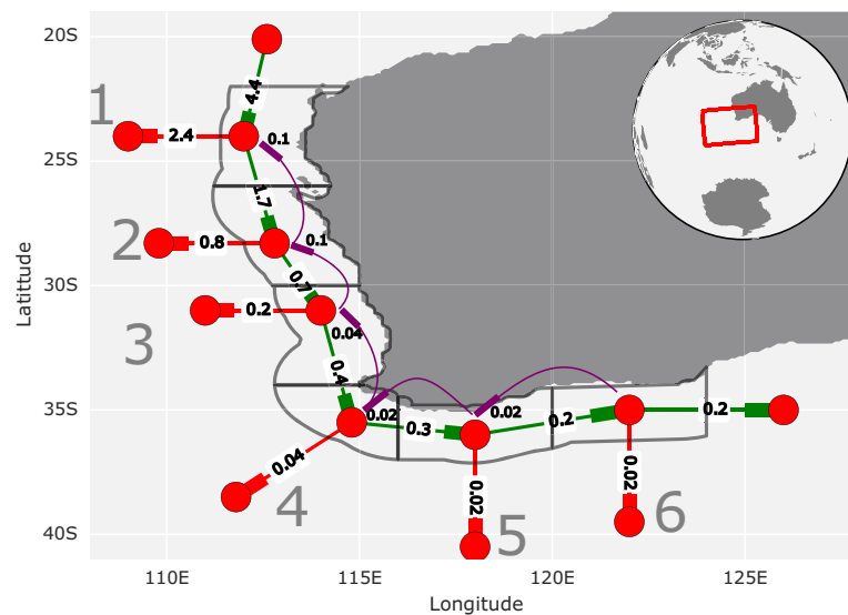
Figure 8. Quantification of direct pathways through the Leeuwin Current region. The bold end of each edge indicates direction of flux. Inshore green edges indicate water that is traveling close to the coast having passed through all preceding inshore sector(s). Offshore red edges quantify trajectories that traveled through all green inshore upstream sector(s) and then exited the system via the red offshore edge. Purple curved edges indicate trajectories that have traveled directly through the previous inshore sector(s) and then recirculated upstream. Units are in Sv and the mean is taken over the years 1966–2003 and depth integrating to 300 m.
