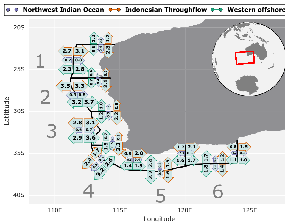
Figure 5. Source water exchange along the Leeuwin Current's pathway. Numbers are transport (Sv) across the pictured sector boundaries (black lines), taking the average for years 1966–2003 and depth-integrating to 300 m. Orange arrows are particles originating from the Indonesian Throughflow region, purple arrows are from the northern offshore section, and green arrows from the western offshore section. Size and direction of arrows are indicative of transport size and direction of flow, respectively.
