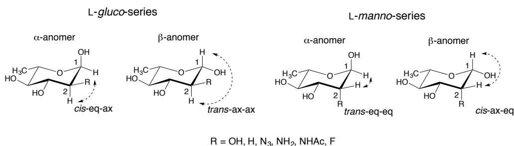
Figure 3: Conformations of 2-substituted L-quinovose and L-rhamnose
