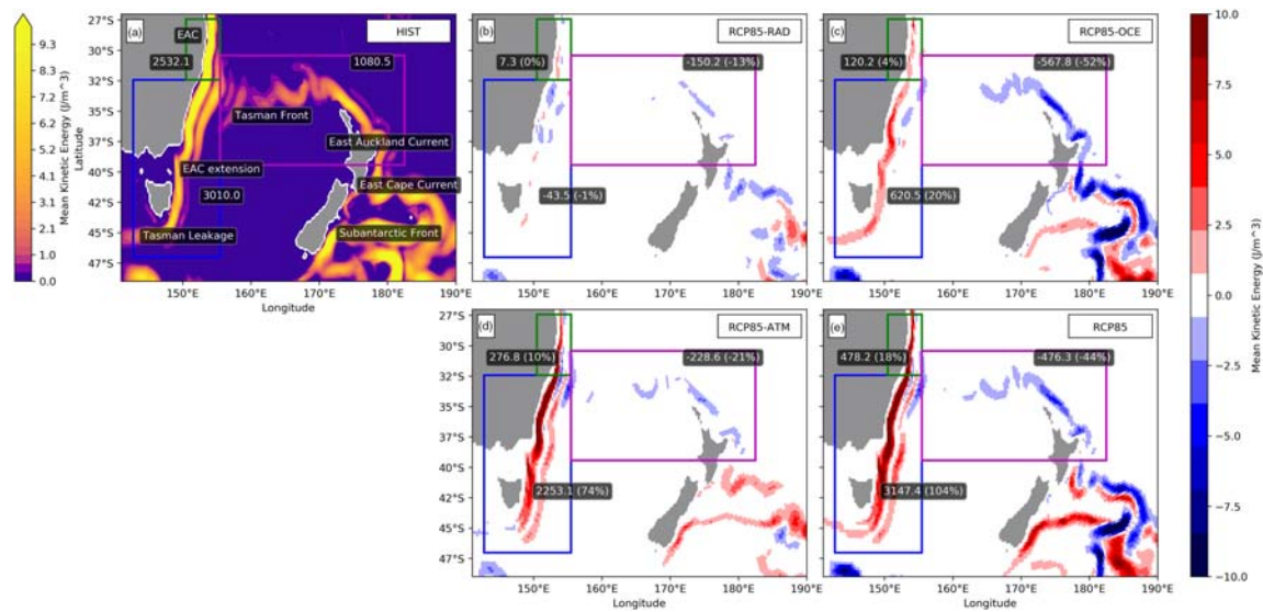
Figure 5. Volume-averaged mean kinetic energy (MKE) for (a) HIST and (b–e) difference from HIST for future climate change scenarios. MKE(x, y) = \frac{\rho_0}{2D} \int_0^D (\bar{u}^2(x, y, z) + \bar{v}^2(x, y, z)) dz , where \bar{u} and \bar{v} are the time-mean horizontal velocity components, \rho_0 = 1035 \text{ kg m}^{-3} , and D is the depth of the seafloor or 1,945 m, whichever is shallower. Highlighted boxes indicate the area used for the total calculated MKE of the following: EAC (green), EAC extension (blue), and Tasman Front (magenta) regions, where (a) total MKE and (b–e) has MKE difference from HIST in \text{J/m}^3 (% change).
