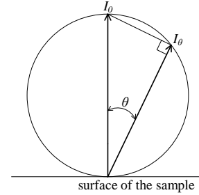
Fig.1 (c) The radiant intensity depends on the direction of emission.
