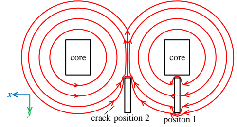
Fig. 4 Eddy currents paths when the crack at different position.
