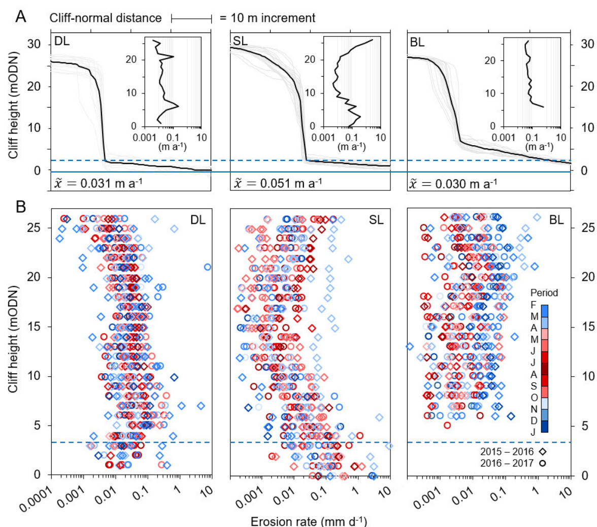
Figure 8. (A): Lithology-specific cliff-normal topographic profiles. Grey lines are individual profiles, extracted every 5 m of cliff line distance for representative sections of each unit. Black line shows mean profile. \tilde{x} = mean erosion rate per lithology. Solid and dashed blue lines indicate position of mean sea level and the highest astronomical tide, respectively. Inset panels show mean erosion rate (x-axis for all = \text{m a}^{-1} ) according to cliff height (y-axis; mODN). DL, SL, and BL are dolomitic,
