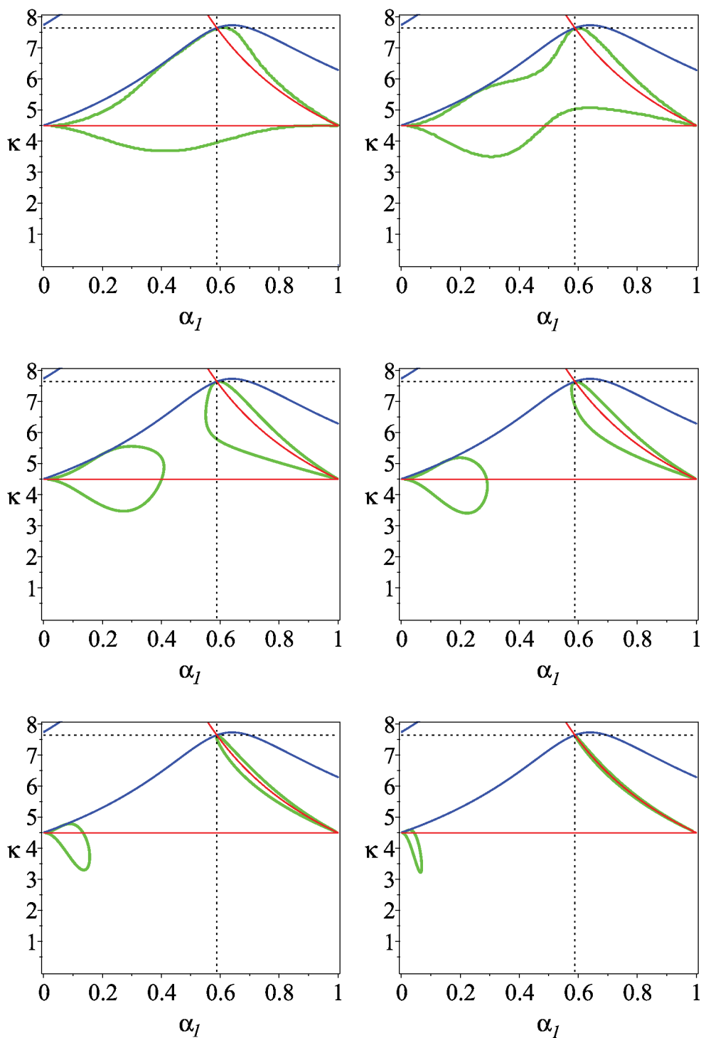
Fig. 7 Stability diagrams in the (\alpha_1, \kappa) -plane for (upper left) \beta_1 = \pi/2 - 0.5 , (upper right) \beta_1 = \pi/2 - 0.15 , (middle left) \beta_1 = \pi/2 - 0.1 , (middle right) \beta_1 = \pi/2 - 0.05 , (lower left) \beta_1 = \pi/2 - 0.01 , and (lower right) \beta_1 = \pi/2 - 0.001 . The black dashed lines intersect at the point with the coordinates of the optimal solution: \alpha_1^* \approx 0.588527598 and \kappa^* \approx 7.635002111 .
