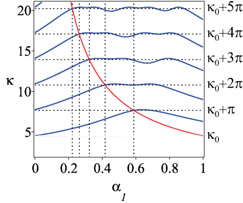
Fig. 9 Graphs of (red) equation (3.6) defining the flutter boundary in the limit \beta_1 = \pi/2 as a function of \alpha_1 and (blue) equation (3.3) defining the divergence boundary as a function of \alpha_1 . The intersection points are given by the expressions (3.9) and (3.10) and listed in Table 1.
