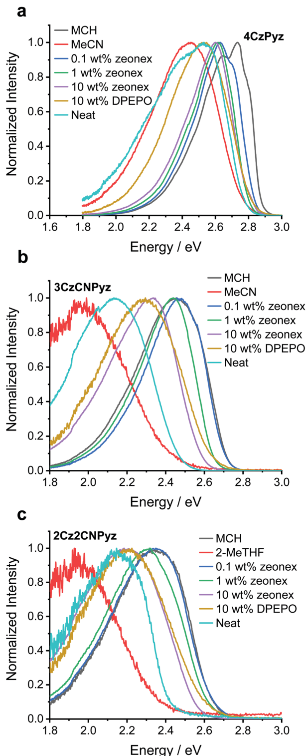
Fig. 2 The photoluminescence of 10 \mu M solutions in methylcyclohexane (MCH) and acetonitrile (MeCN), doped zeonex and DPEPO films and neat films of (a) 4CzPyz (b) 3CzCNPz and (c) 2Cz2CNPz . [N.B. For 2Cz2CNPz 2-MeTHF replaces MeCN as negligible signal-to-noise ratio was observed in the MeCN sample, most likely a result of severe relaxation of the CT state and associated increase in non-radiative decay].
