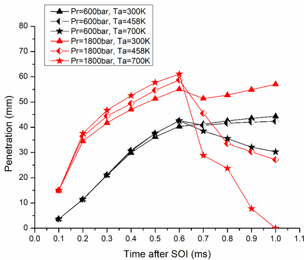
11 Fig. 9. Effect of ambient temperature on spray tip penetration when T_f=387\text{K} and P_a=26\text{ bar}
