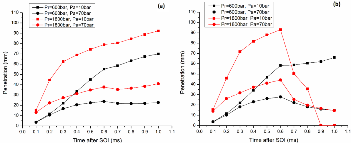
8 Fig. 8. Effect of ambient pressure on spray tip penetration
