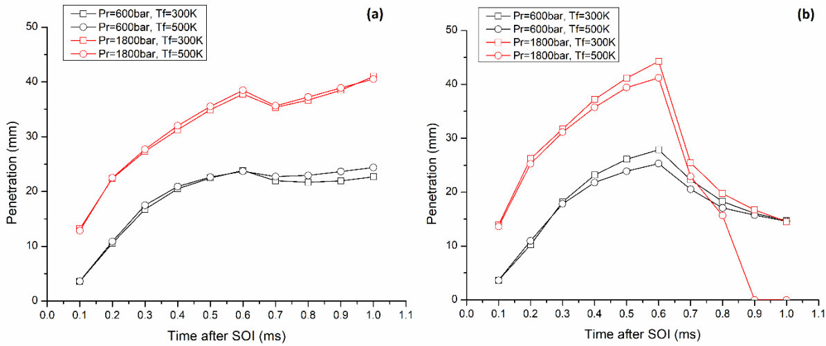
Fig. 11. Effect of fuel temperature on spray tip penetration
