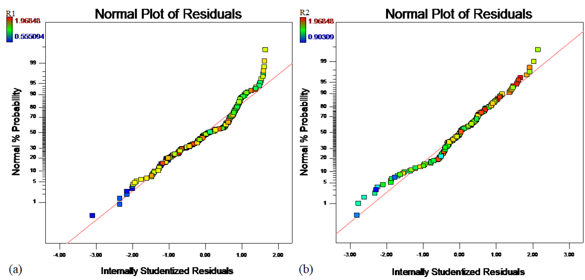
12 Fig. 12. Normal probability plots of residuals for R1 (a) and R2 (b)
