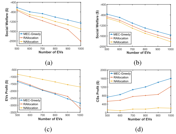
Fig. 5. Social welfare with (a) 50% and (b) 100% V2G penetration. Profit for (c) EVs and (d) CSs with 50% V2G penetration.
