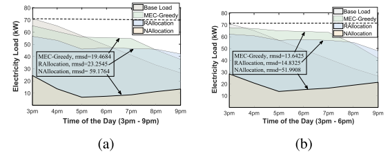
Fig. 9. Load shifting: (a) 20% and (b) 25% charging penetration.
