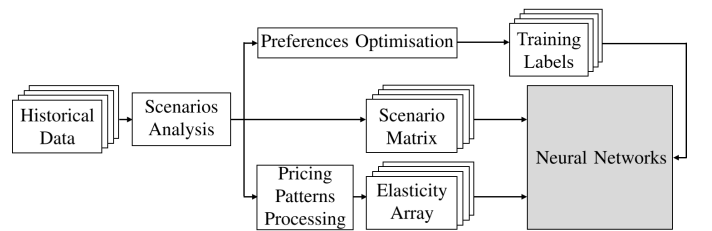
Fig. 2. Flowchart of the training phase of the energy scheduling model. Historical data is processed by the scenarios analysis and pricing patterns processing approaches as training inputs of developed neural networks. The training labels are optimal scheduling decisions yielded by solving the preferences optimisation problems.
