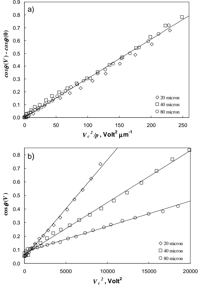
FIG. 4. (a) Data for three electrode pitches (20, 40 and 80 μm) plotted as a function of the effective voltage normalized by electrode mechanical pitch. The effective voltage takes into account the capacitive division caused by the solid dielectric layer on the interdigitated electrodes. (b) Data presented showing the effect of reducing the electric potential penetration depth into the liquid caused by changing the electrode mechanical pitch.
