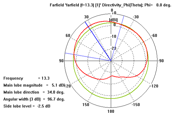
Figure 9-b. Resultant H-plane pattern for perpendicular polarisation
