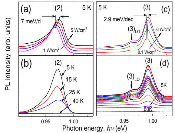
Fig. 2. Excitation intensity dependence of the type (2) PL spectra (a), temperature dependence of the type (2) PL spectra (b), excitation intensity dependence of the type (3) PL spectra (c), temperature dependence of the type (3) PL spectra (d).
