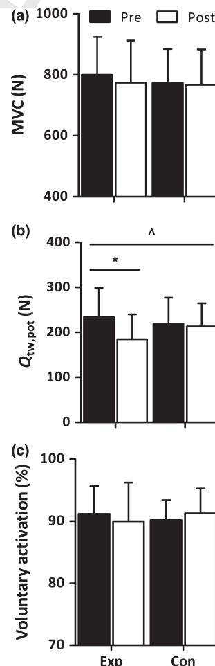
Fig. 3. Maximum voluntary contraction force (a), potentiated twitch force (b) and voluntary activation (c) pre and post low-volume, heavy-resistance exercise (Exp), and at the same time points in a control condition of passive rest (Con). *Different to pre-, ^Significant interaction effect ( P < 0.05 ).
