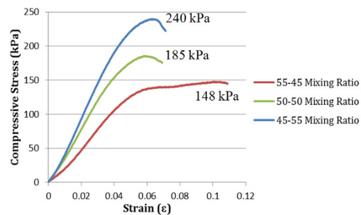
Fig. 6. Compressive stress strain curves for different mixing ratios
