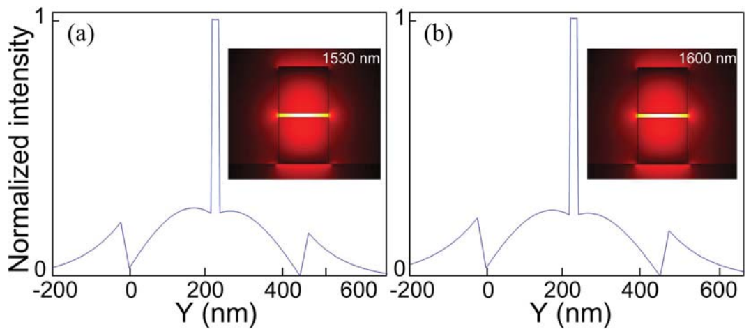
Figure 4. Normalized power density of the quasi-TM polarization of (a) probe and (b) pump. The insets illustrate the corresponding transverse profiles of the electric field for the quasi-TM polarization.
