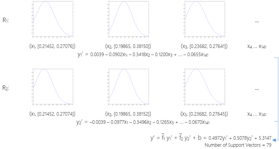
Figure 3: Illustration of the TSK-SVR model and its parameters for Task 4 with two rules. As this has 141 features and is not possible to fit in the paper, only the first three normalised features were presented. The rules should be read using IF before each feature’s membership function, AND between the features, and finally THEN before the consequent part is defined. The Gaussian membership function parameters were specified by two parameters (i.e., [standard deviation, mean]). Number of support vectors that determines the coefficients of linear expression ( w and b ) is 79.
