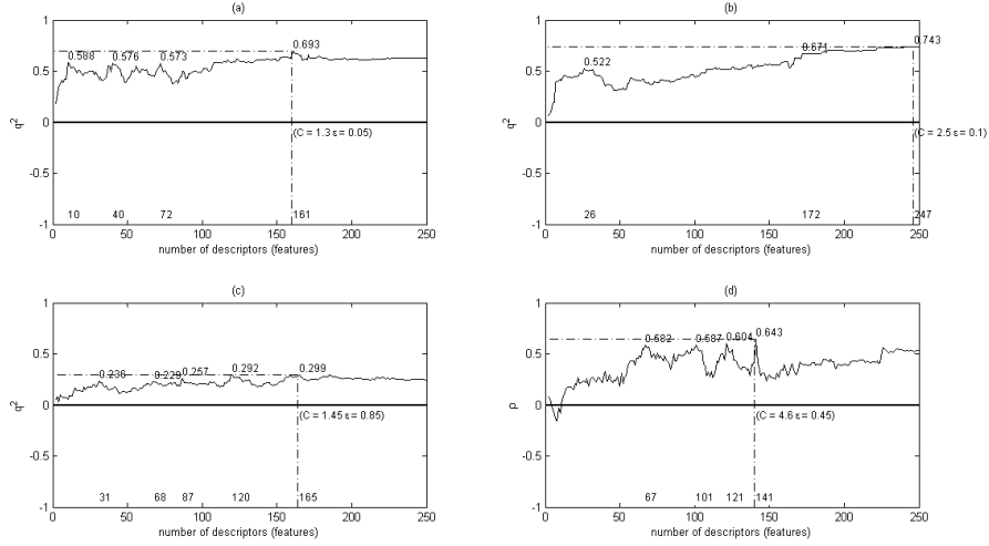
Figure 6: The performance of 4-rule fuzzy model based on the number of descriptors. a) Task 1: Graph reaches highest peak at 161 with the SVR parameters ( C = 1.3 and \epsilon = 0.05 ). b) Task 2: Graph reaches highest peak at 247 with the SVR parameters ( C = 2.5 and \epsilon = 0.1 ). c) Task 3: Graph reaches highest peak at 165 with the SVR parameters ( C = 1.45 and \epsilon = 0.85 ). d) Task 4: Graph reaches highest peak at 141 with the SVR parameters ( C = 4.6 and \epsilon = 0.45 ).
