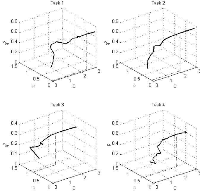
Figure 2: Illustration of grid-search for TSK-SVR to find the optimum values of parameters ( C and \epsilon ) and prediction performance ( q^2 or \rho ) based on the selected features for the peptide binding affinity Tasks 1-4. For simplicity, the grid-search iterates C parameter with a step size 0.05 in the range 0.05-3.00 while \epsilon remained fixed. a) Task 1 with seven rules and 161 features yielded a q^2 value of 0.696 with SVR parameters C = 2.4 and \epsilon = 0.05 . b) Task 2 with three rules and 247 features yielded a q^2 value of 0.743 with SVR parameters C = 1.9 and \epsilon = 0.10 . c) Task 3 with three rules and 172 features yielded a q^2 value of 0.310 with SVR parameters C = 1.45 and \epsilon = 0.90 . d) Task 4 with two rules and 141 features yielded a \rho value of 0.643 with SVR parameters C = 2.3 and \epsilon = 0.45 .
