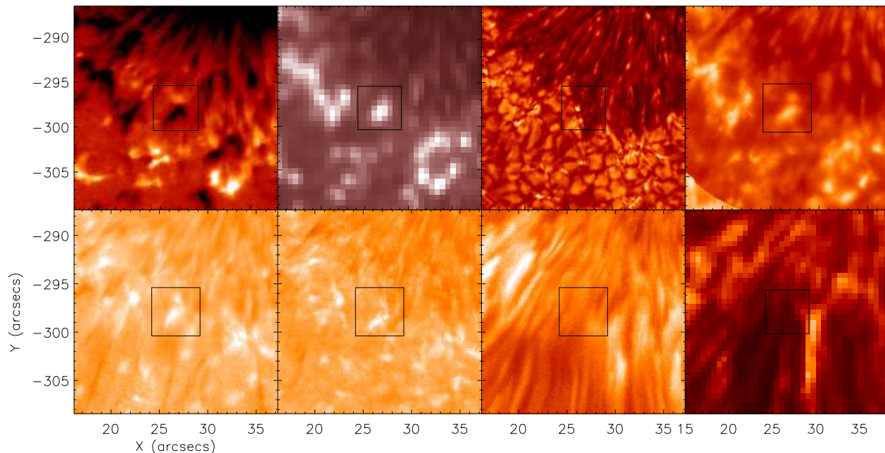
FIG. 1.— (Top row - left to right) Coaligned Hinode/SOT Stokes V/I, SDO/AIA 1700 Å, ROSA G-band, and IBIS Fe I line core. (Bottom row - left to right) IBIS H \alpha blue and red wing images (approximately \pm 0.75 Å), IBIS H \alpha line core, and SDO/AIA 304 Å. A box including the event analysed in Fig. 3, Fig 6, and Fig. 7 is overlotted. This FOV is taken at the temporally closest image for each wavelength to 14:56:35 UT.
