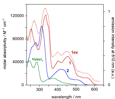
Fig. 2 Absorption spectra of 1 (red solid line), 2 (blue) and fac -Ir(ppy) 3 (green) in CH 2 Cl 2 at 298 ± 3 K. The excitation spectrum of 1 under the same conditions, registered at \lambda_{\text{em}} = 610 \text{ nm} , is the red dotted line labelled 1ex .
