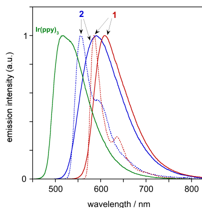
Fig. 3 Emission spectra of 1 , 2 and fac -Ir(ppy) 3 in CH 2 Cl 2 at 298 ± 3 K (red, blue and green solid lines respectively), together with the spectra of 1 and 2 at 77 K in diethyl ether / isopentane / ethanol (2:2:1 v/v).
