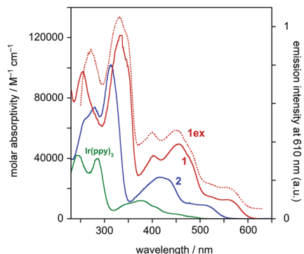
Fig. 2 Absorption spectra of 1 (red solid line), 2 (blue) and fac -Ir(ppy) 3 (green) in CH 2 Cl 2 at 298 ± 3 K. The excitation spectrum of 1 under the same conditions, registered at λ em = 610 nm, is the red dotted line labelled 1ex .
