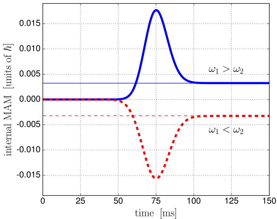
FIG. 2. (Color online) Internal MAM (in units of \hbar ) as a function of propagation time (in milliseconds) in a tilted ridge barrier system. The parameters of the system are as follows: V_0 = 10^{-14} eV, \ell = 20 \mu\text{m} , \mu = 7.016003 u ( {}^7\text{Li} atom), q = 0.3 mm, and v = 4 mm/s. The (blue) thick solid curve represents the case of \omega_1 = 10 s ^{-1} and \omega_2 = 5 s ^{-1} , and the (blue) thin solid line shows the corresponding value of [\Delta\mathcal{L}_i]_3 , as predicted by Eq. (78). The (red) thick dashed curve represents the case of \omega_1 = 5 s ^{-1} and \omega_2 = 10 s ^{-1} , and the (red) thin dashed line shows the corresponding value of [\Delta\mathcal{L}_i]_3 , as predicted by Eq. (78).
