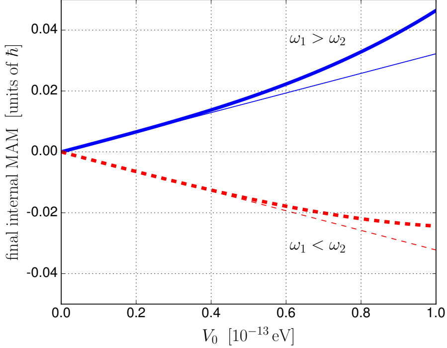
FIG. 3. (Color online) Internal MAM (in units of \hbar ) at time t = 150 ms, at which the wave packet is located to the right of the barrier (cf. Fig. 2), as a function of the potential strength (in units of 10^{-13} eV). All parameter values are the same as in Fig. 2. The (blue) thick solid curve represents the case of \omega_1 = 10 \text{ s}^{-1} and \omega_2 = 5 \text{ s}^{-1} , and the (blue) thin solid line shows the corresponding value of [\Delta\mathcal{L}_i]_3 , as predicted by Eq. (78). The (red) thick dashed curve represents the case of \omega_1 = 5 \text{ s}^{-1} and \omega_2 = 10 \text{ s}^{-1} , and the (red) thin dashed line shows the corresponding value of [\Delta\mathcal{L}_i]_3 , as predicted by Eq. (78).
