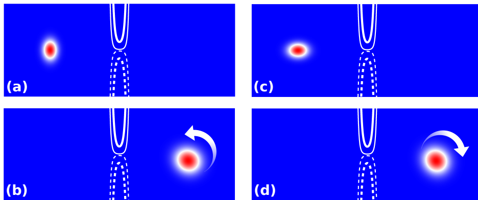
FIG. 1. (Color online) An illustration of a Gaussian wave packet passing over the tilted ridge barrier, defined by Eqs. (58) and (79). Four white curves show equipotential curves: the solid (dashed) curves correspond to positive (negative) values of the potential; the curve thickness increases as the absolute value of the potential becomes larger. The wave packet travels from left to right. (a) and (b) show the initial and final probability densities, respectively, for the case of \omega_1 > \omega_2 . (c) and (d) is the corresponding pair of figures in the case of \omega_1 < \omega_2 . The curly arrows in (b) and (d) show the sense of the internal rotation of the final wave packet.
