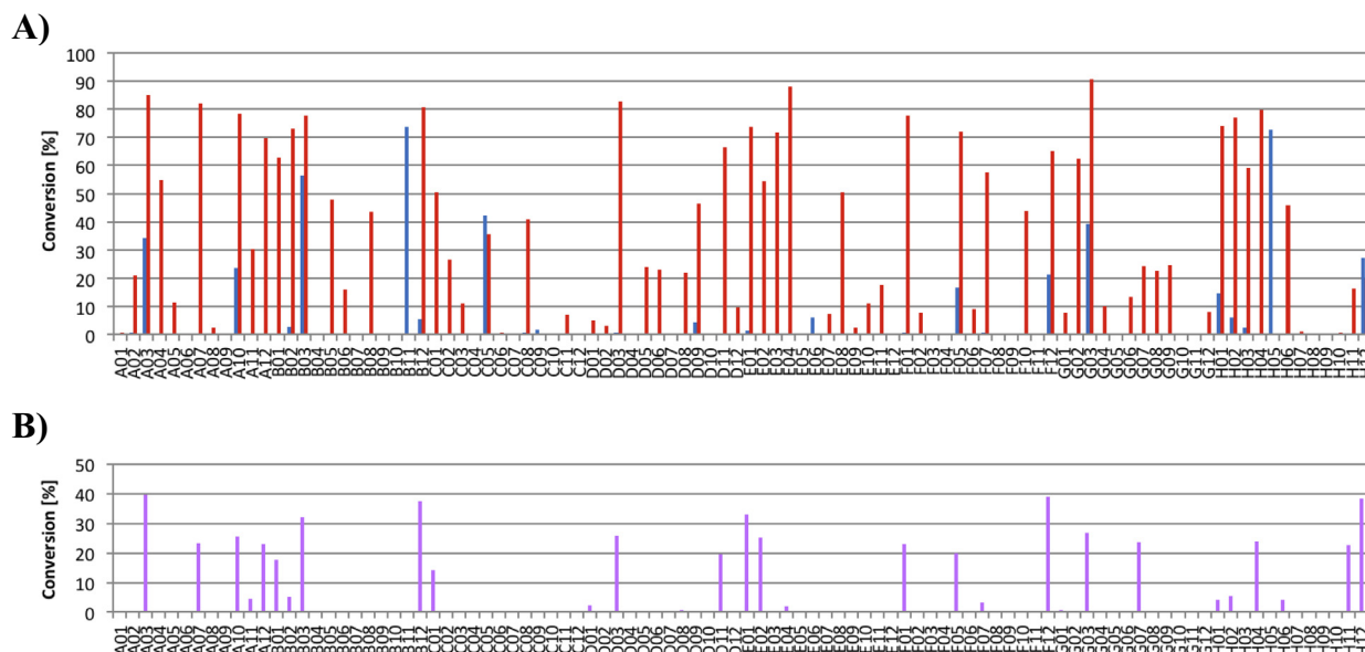
Fig. 2. A) Exemplary screening of a highly diverse metagenomic short-chain dehydrogenase/reductase (SDR) array in 96-well plate format (Prozomix Ltd, Cat No. PRO-KRED (00289–00384)), by using individual enantiomers ( S )- 1a and ( R )- 1a (■ and ■, respectively). Maximum substrate conversion after 1.5 h was 90% as determined by comparison against a fluorescence standard curve measured with ketone 2a under identical assay conditions. B) Screening of the same plate by using rac - 1b as substrate (■).
