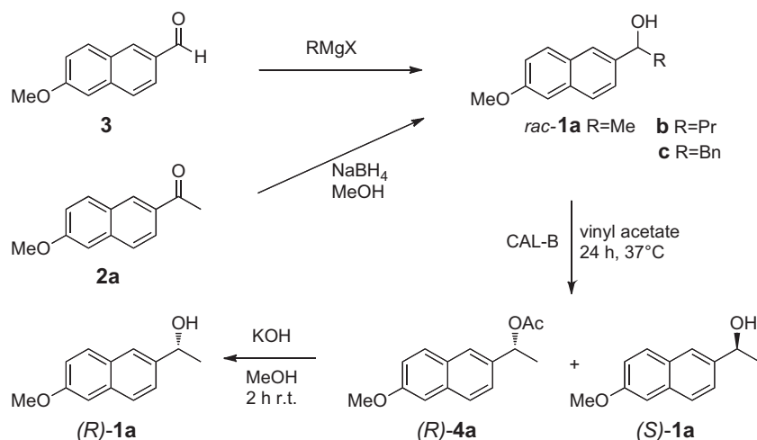
Scheme 2. Synthesis of substrate alcohols 1a–c and racemate resolution of 1a by lipase catalyzed transacylation.
