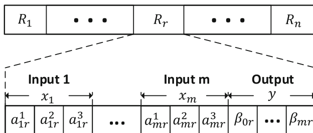
Fig. 3 Chromosome encoding
