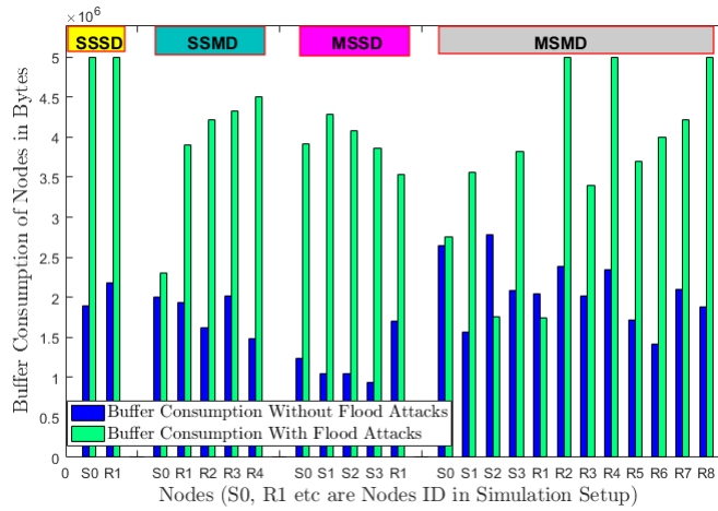
Fig. 15. Impact of Flood attacks on Buffer Consumption
