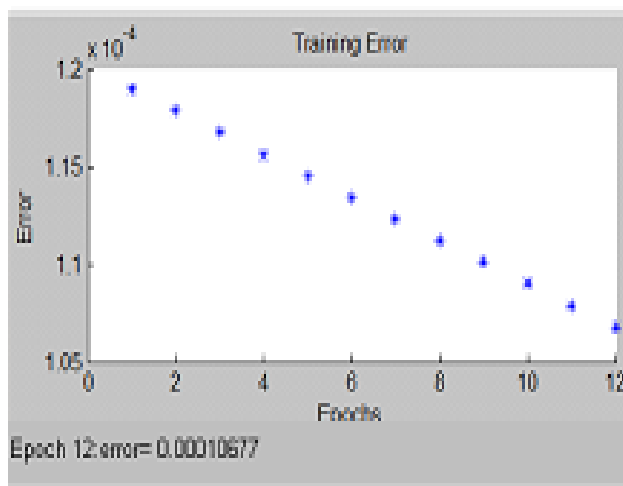
Fig. 6. Training result
