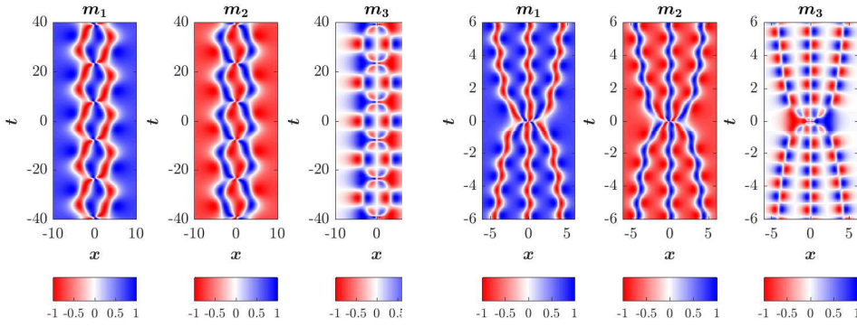
(a) Stationary, breather-like soliton
