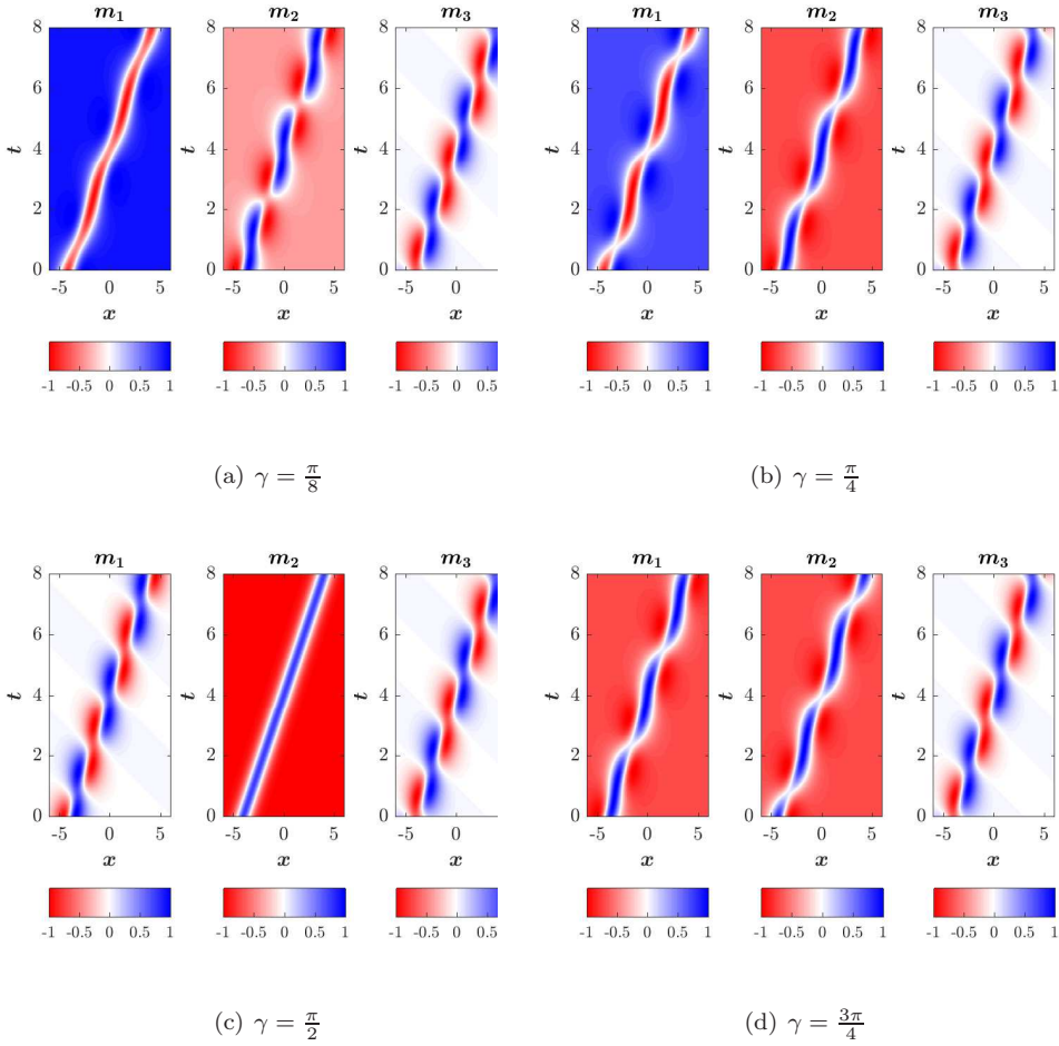
Fig. 1 Propagating, one-soliton solution, for different values of the asymptotic angle \gamma .
