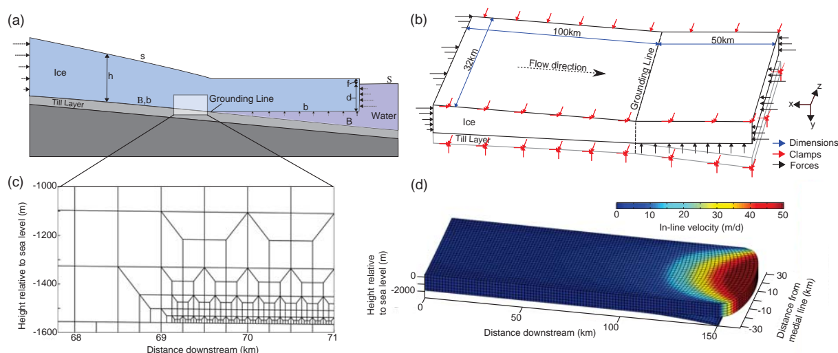
Figure 1. Model setup for 2-D ( a , c ) and 3-D ( b , d ) simulations. Panels ( a ) and ( b ) are schematic representations of the model domains while ( c ) and ( d ) show the model grid (panel ( c ) is zoomed in to show refinement near the grounding line). The 3-D grid in ( d ) has been vertically exaggerated by a factor of 4.
