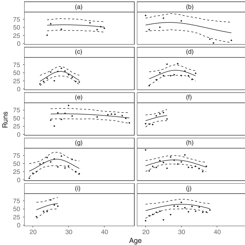
Fig. 5. Posterior mean and central 95% bands for the aging profile (1 - \pi_i) \exp\{\theta_i + f_i(a)\} of various batsmen together with their posterior mean-adjusted runs scored: (a) A. D. Nourse; (b) G. A. Headley; (c) H. H. Gibbs; (d) H. M. Amia; (e) J. B. Hobbs; (f) K. S. Williamson; (g) M. D. Crowe; (h) R. T. Ponting; (i) S. P. D. Smith; (j) S. R. Waugh
