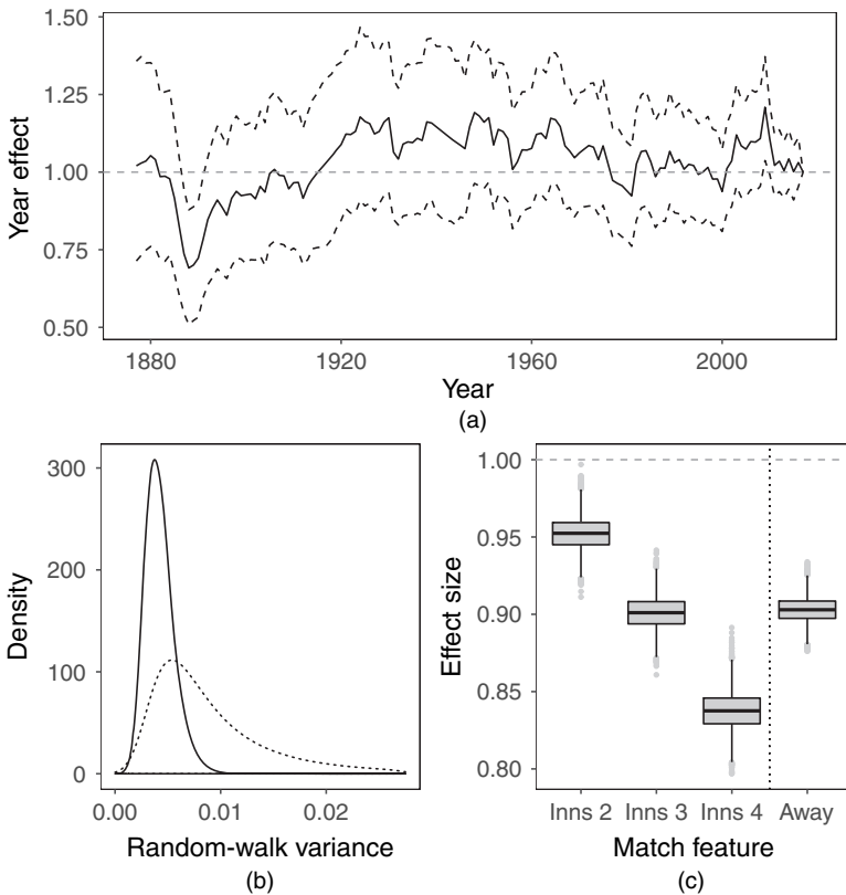
Fig. 3. (a) Posterior mean and central 95% bands for the multiplicative year effects \exp(\delta_t) , (b) posterior (—) and prior (-----) density plots for the smoothing parameter \sigma_\delta^2 and (c) boxplots of the posterior distributions for the multiplicative match innings effects \exp(\nu_m) and playing away effect \exp(\zeta_2)
