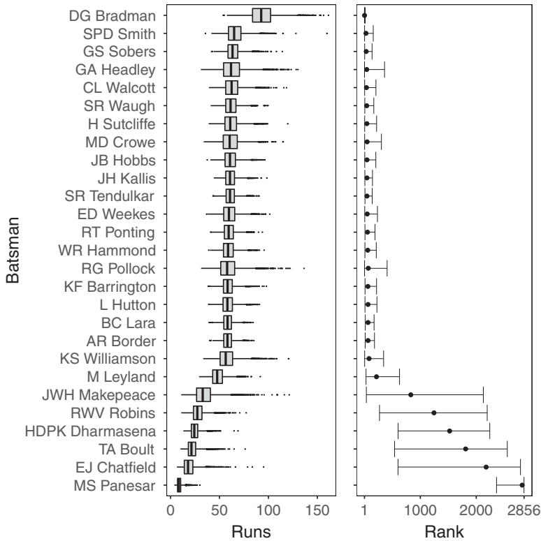
Fig. 6. Posterior distributions of some players' abilities \exp(\theta_i) and their ranking confidence intervals
