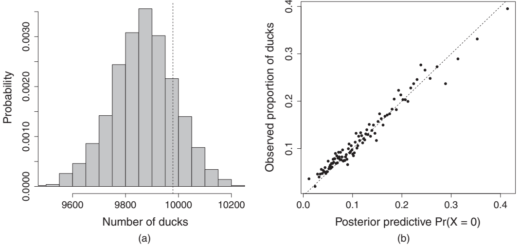
Fig. 7. (a) Posterior predictive distribution of total ducks ( \cdot , observed number in the data) and (b) observed proportion of ducks against centiles of posterior predictive probabilities of a duck
