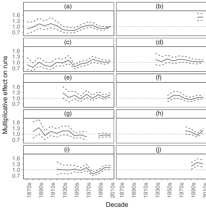
Fig. 4. Posterior mean and central 95% bands for the multiplicative opposition effects by decade, \exp(\xi_q + \omega_{qd}) : (a) Australia; (b) Bangladesh; (c) England; (d) India; (e) New Zealand; (f) Pakistan; (g) South Africa; (h) Sri Lanka; (i) West Indies; (j) Zimbabwe
