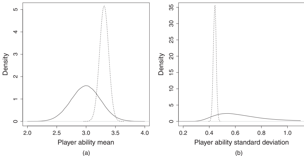
Fig. 2. Prior (—) and posterior (-----) density plots for ability parameters (a) \mu_\theta and (b) \sigma_\theta
