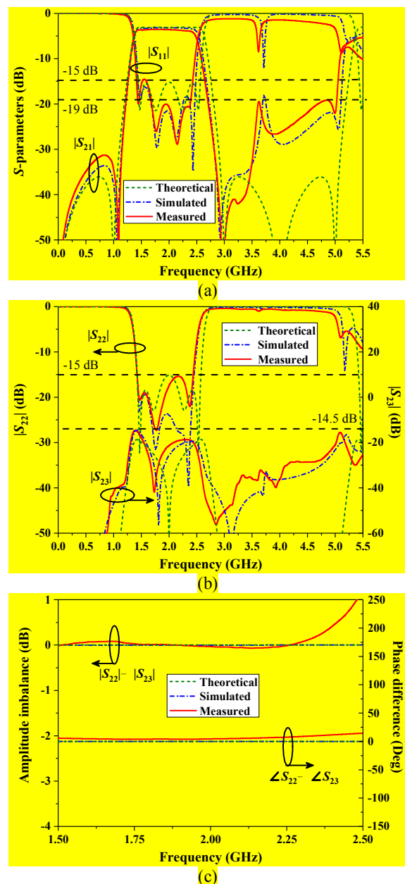
Fig. 7. The theoretical, EM simulated and measured results of the proposed bandpass FPD: (a) S_{11} and S_{21} , (b) S_{22} and S_{23} , and (c) phase imbalance and amplitude imbalance.
