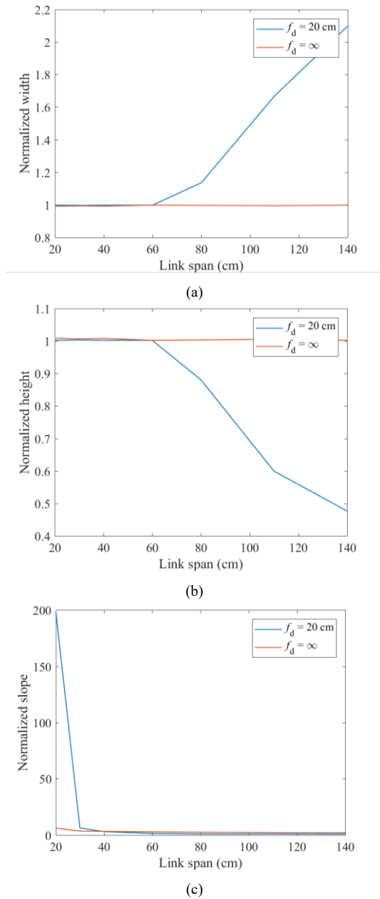
Fig. 8. Normalized parameters of the image of a LS against link span camera focused at 20 cm and infinity, the LS aperture diameter of 3 cm, and the camera lens f-stop of 5.6 for: (a) width, (b) height, and (c) slope.
