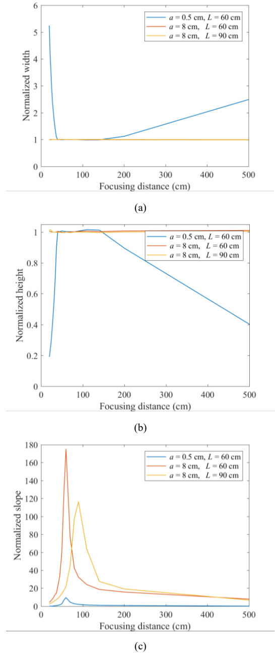
Fig. 7. Normalized values of the image of a LS vs. focusing distances for LS apertures of 0.5 cm, 8 cm, and 8 cm at L of 60 cm, 60cm and 90 cm, respectively and a lens f-stop was 5.6 for (a) width, (b) height, and (c) slope.
