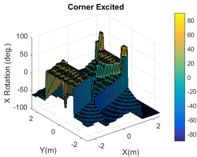
Fig. 7- Rotation angle limit in x-z plane for corner excited Tx pattern
