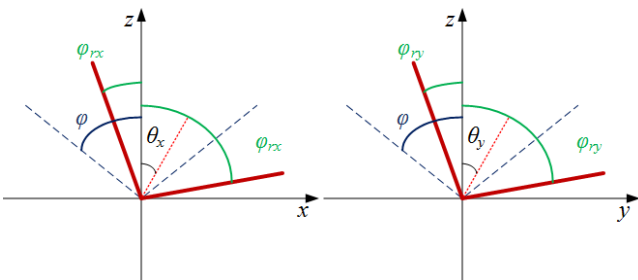
Fig. 2- The Rx rotation in the x - z and y - z planes
