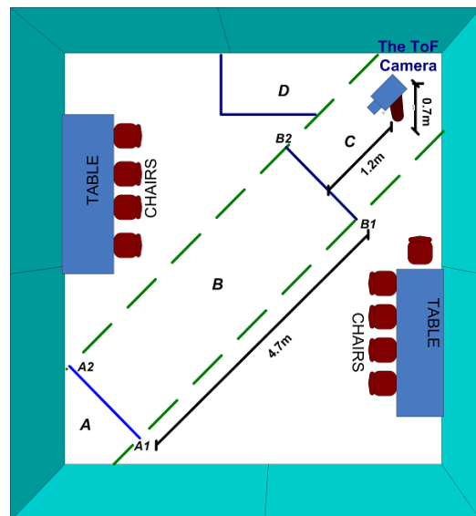
Fig. 1. Aerial view of the gait image sequence capture setup of the proposed frontal view gait data set using the ToF camera.
