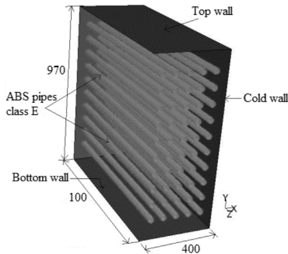
Figure 1: configuration of the flow domain (all dimension are in mm)
