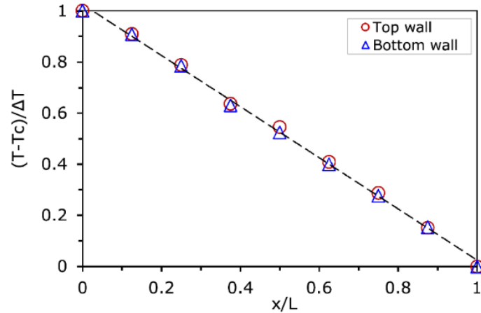
Figure 5: Temperature profile on horizontal walls
