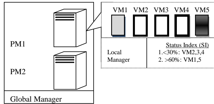
Figure 1. Local Manager with Status Index that keeps record of CPU utilization percentage of VMs
