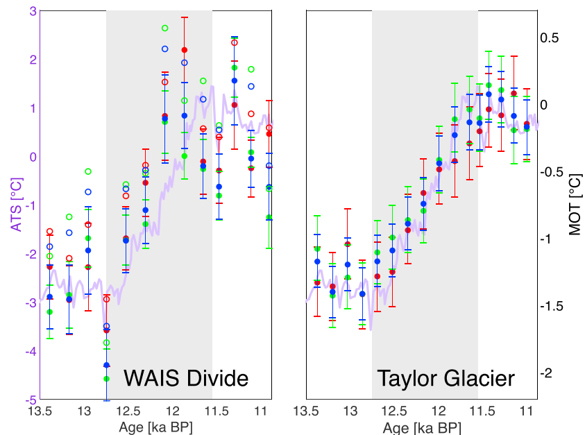
Figure 1. Mean ocean temperature (MOT) records for published WAIS Divide (WD; left; Bereiter, Shackleton, et al., 2018) and Taylor Glacier (right) derived from \text{Kr}/\text{N}_2 (red), \text{Xe}/\text{N}_2 (blue), and \text{Xe}/\text{Kr} (green) with 1\sigma uncertainties (scale on right). Open circles in left panel show WD data corrected with the least squares method applied in this study. Antarctic temperature stack (ATS; Parrenin et al., 2013) is shown in purple (scale on left). MOT and ATS data are displayed as anomalies relative to modern. Gray bars highlight the Younger Dryas.
